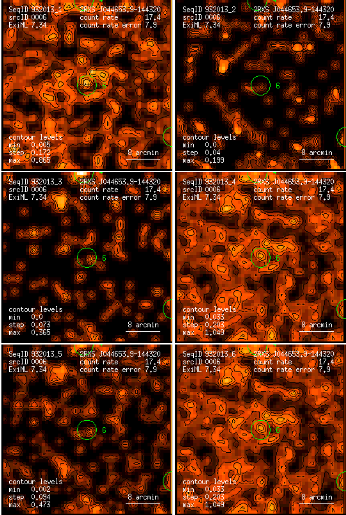
Figure 6: RASS 932013: detection 0006: band rate images, Gaussian filter: (1) PSPC channels 11 – 41, (2) 52 – 90, (3) 91 – 201, (4) 11 – 235, (5) 52 – 201, (6) 11 – 201. Broad band rates in counts/ks. Band rate contour levels in counts/ks/arcmin 2 .
