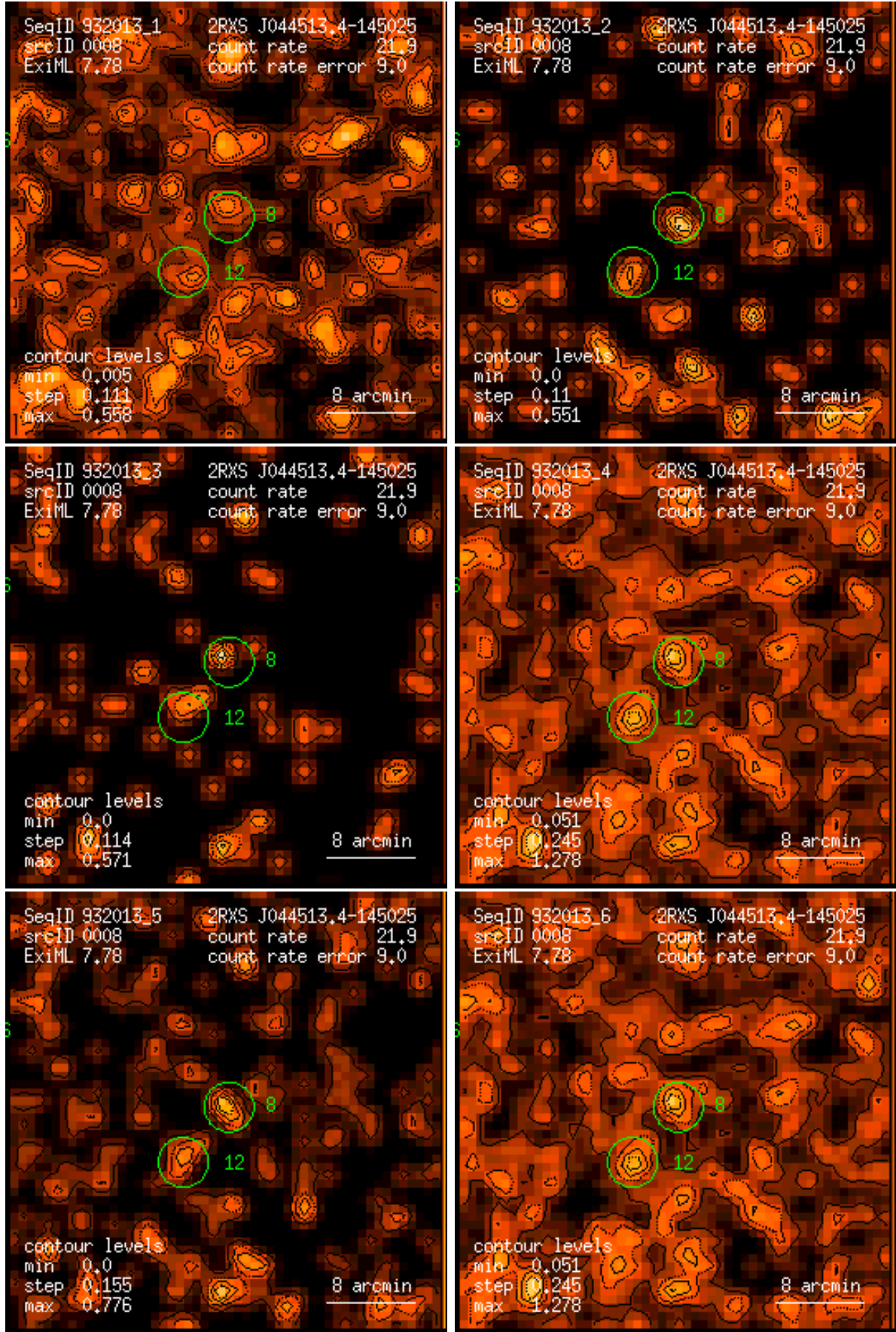
Figure 8: RASS 932013: detection 0008: band rate images, Gaussian filter: (1) PSPC channels 11 – 41, (2) 52 – 90, (3) 91 – 201, (4) 11 – 235, (5) 52 – 201, (6) 11 – 201. Broad band rates in counts/ks. Band rate contour levels in counts/ks/arcmin 2 .
