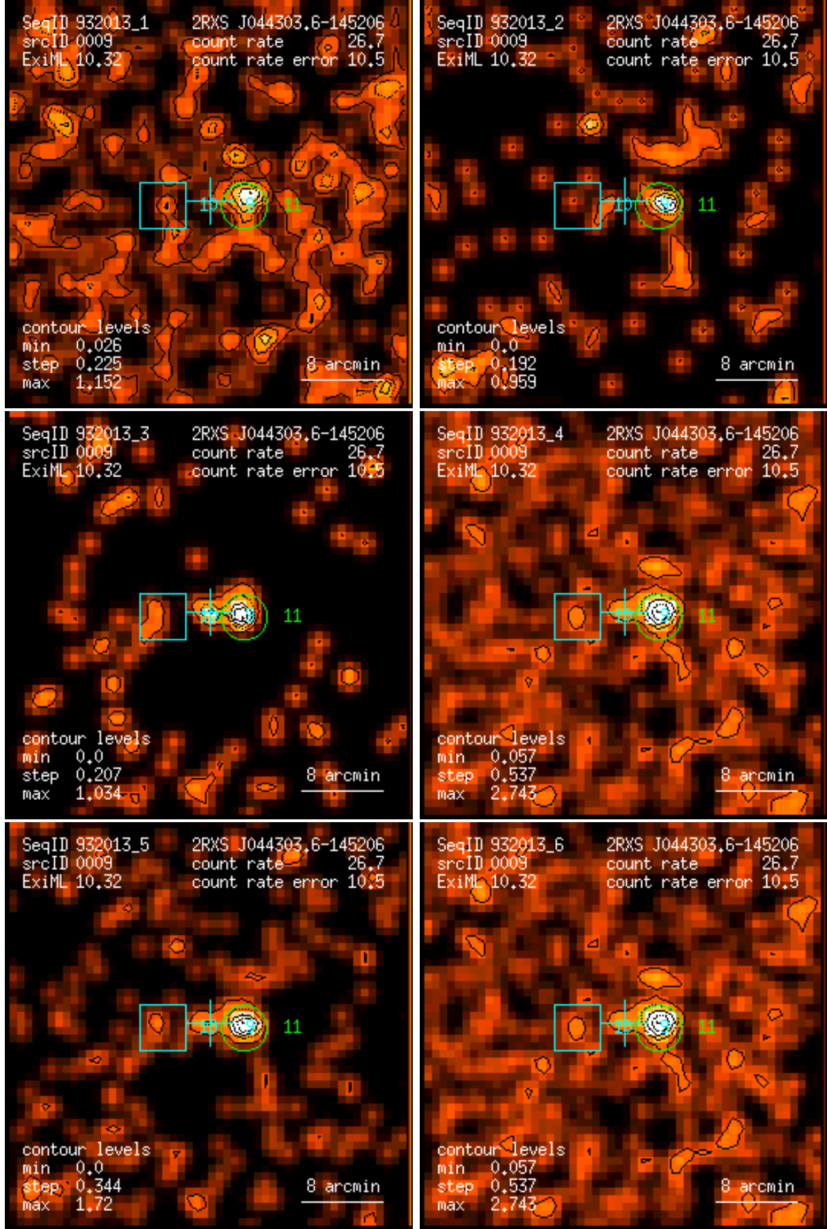
Figure 9: RASS 932013: detection 0009: band rate images, Gaussian filter: (1) PSPC channels 11 – 41, (2) 52 – 90, (3) 91 – 201, (4) 11 – 235, (5) 52 – 201, (6) 11 – 201. Broad band rates in counts/ks. Band rate contour levels in counts/ks/arcmin 2 .
