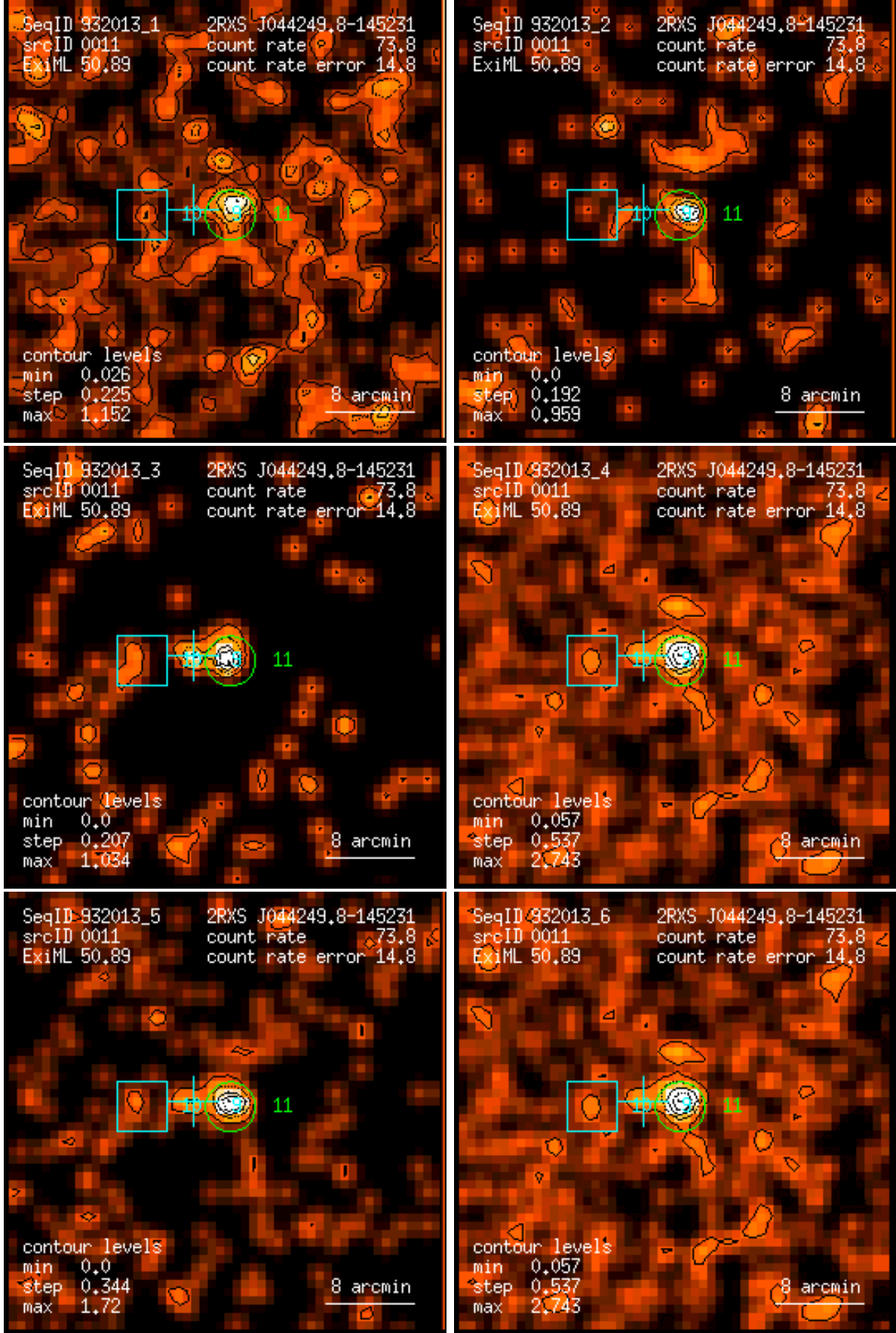
Figure 11: RASS 932013: detection 0011: band rate images, Gaussian filter: (1) PSPC channels 11 – 41, (2) 52 – 90, (3) 91 – 201, (4) 11 – 235, (5) 52 – 201, (6) 11 – 201. Broad band rates in counts/ks. Band rate contour levels in counts/ks/arcmin 2 .
