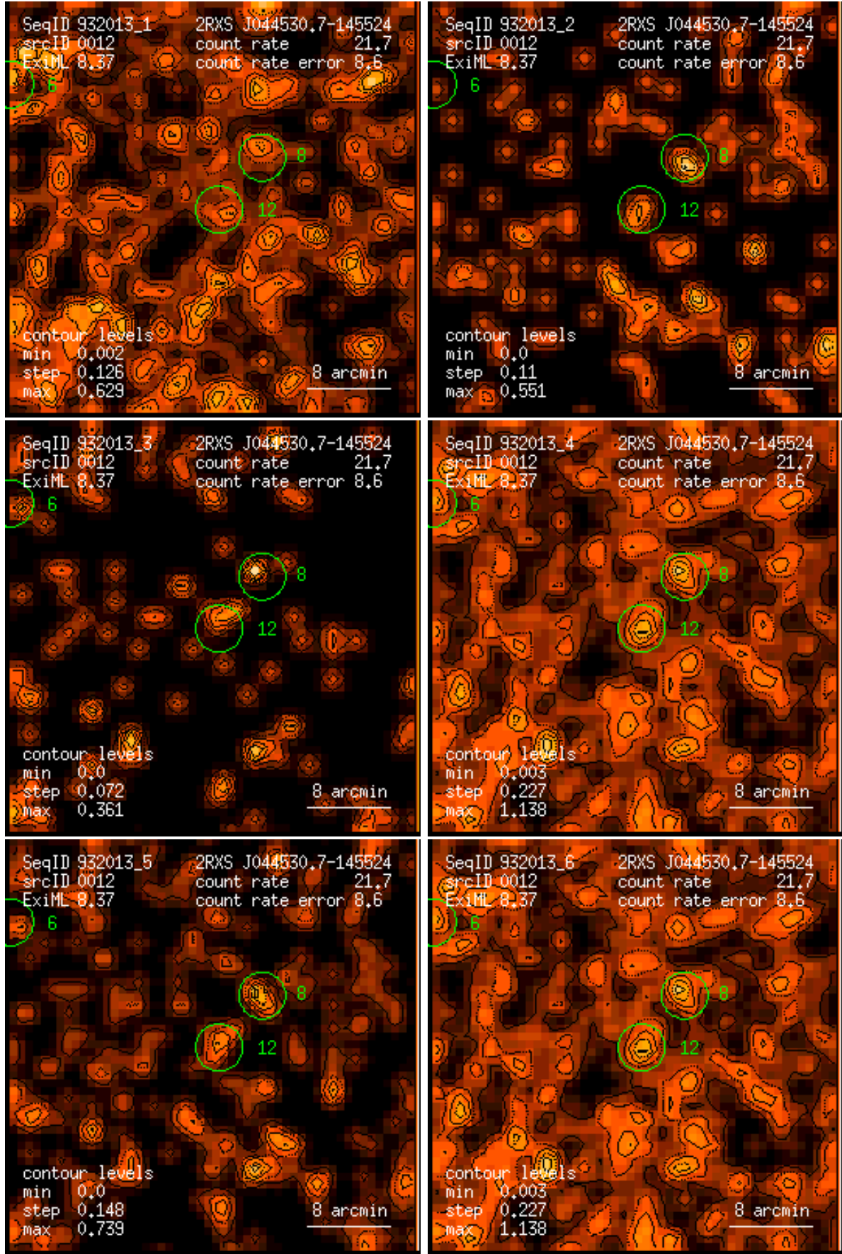
Figure 12: RASS 932013: detection 0012: band rate images, Gaussian filter: (1) PSPC channels 11 – 41, (2) 52 – 90, (3) 91 – 201, (4) 11 – 235, (5) 52 – 201, (6) 11 – 201. Broad band rates in counts/ks. Band rate contour levels in counts/ks/arcmin 2 .
