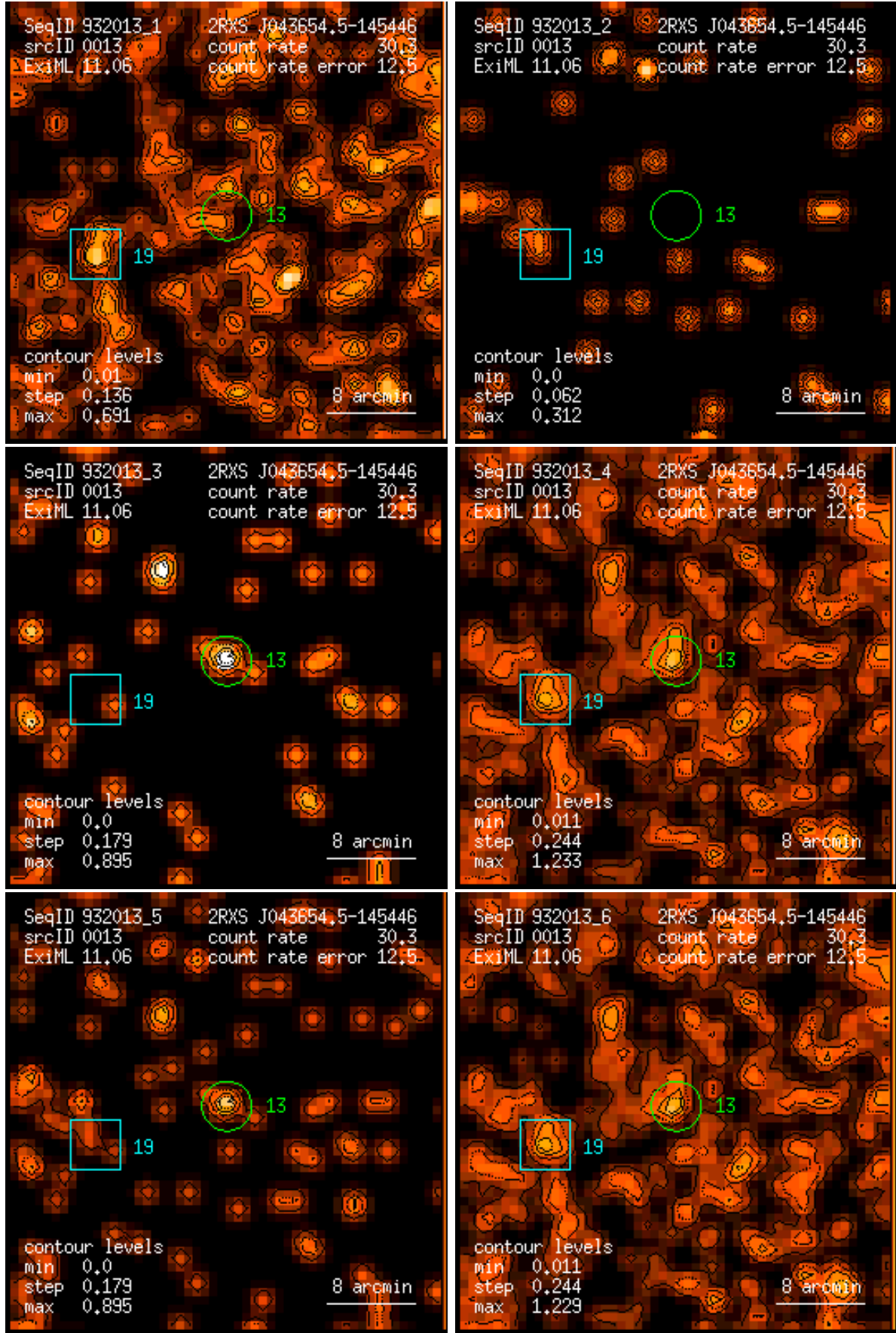
Figure 13: RASS 932013: detection 0013: band rate images, Gaussian filter: (1) PSPC channels 11 – 41, (2) 52 – 90, (3) 91 – 201, (4) 11 – 235, (5) 52 – 201, (6) 11 – 201. Broad band rates in counts/ks. Band rate contour levels in counts/ks/arcmin 2 .
