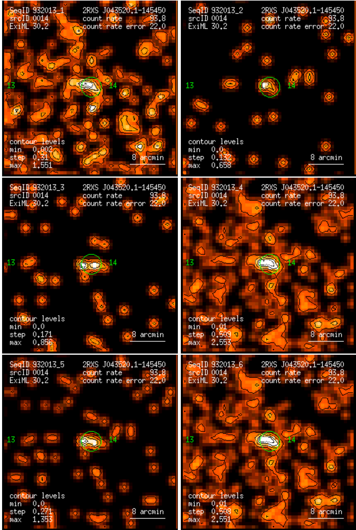
Figure 14: RASS 932013: detection 0014: band rate images, Gaussian filter: (1) PSPC channels 11 – 41, (2) 52 – 90, (3) 91 – 201, (4) 11 – 235, (5) 52 – 201, (6) 11 – 201. Broad band rates in counts/ks. Band rate contour levels in counts/ks/arcmin 2 .
