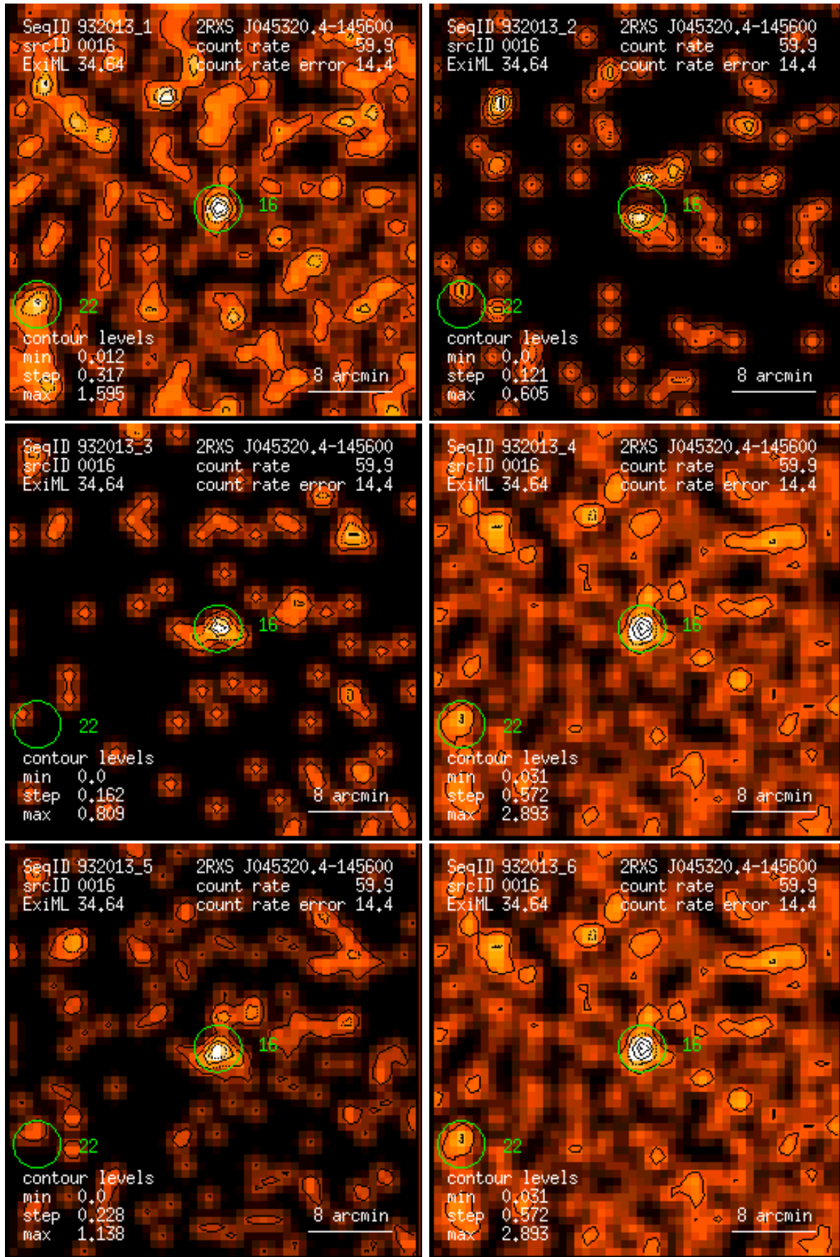
Figure 16: RASS 932013: detection 0016: band rate images, Gaussian filter: (1) PSPC channels 11 – 41, (2) 52 – 90, (3) 91 – 201, (4) 11 – 235, (5) 52 – 201, (6) 11 – 201. Broad band rates in counts/ks. Band rate contour levels in counts/ks/arcmin 2 .
