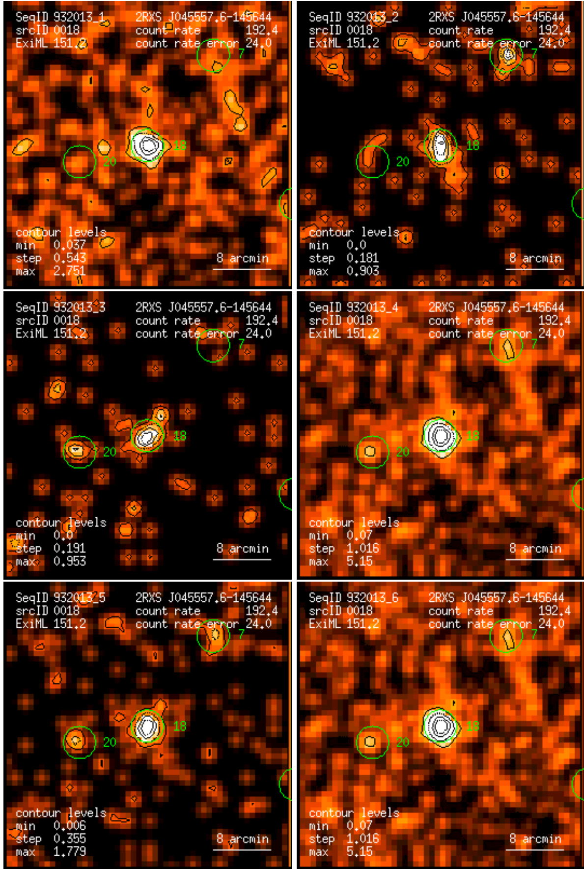
Figure 18: RASS 932013: detection 0018: band rate images, Gaussian filter: (1) PSPC channels 11 – 41, (2) 52 – 90, (3) 91 – 201, (4) 11 – 235, (5) 52 – 201, (6) 11 – 201. Broad band rates in counts/ks. Band rate contour levels in counts/ks/arcmin 2 .
