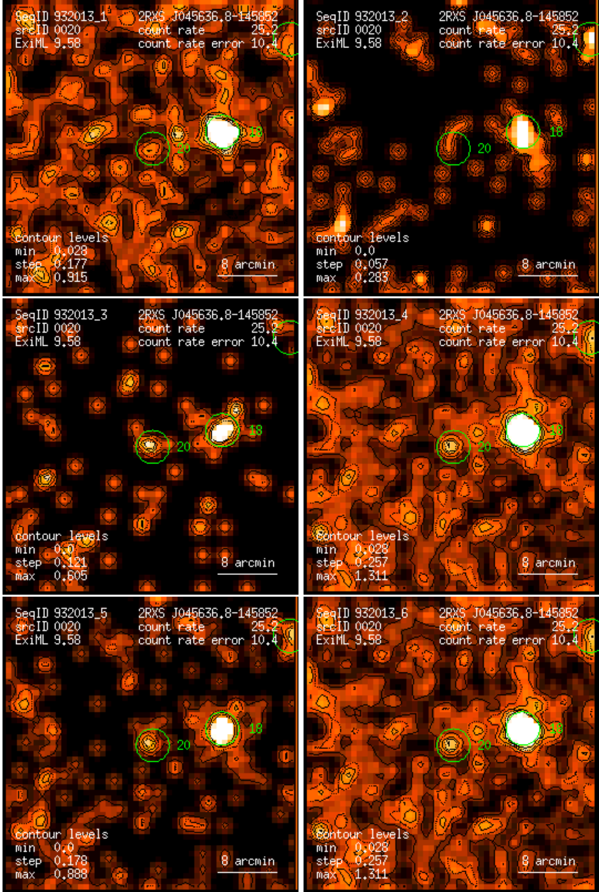
Figure 20: RASS 932013: detection 0020: band rate images, Gaussian filter: (1) PSPC channels 11 – 41, (2) 52 – 90, (3) 91 – 201, (4) 11 – 235, (5) 52 – 201, (6) 11 – 201. Broad band rates in counts/ks. Band rate contour levels in counts/ks/arcmin 2 .
