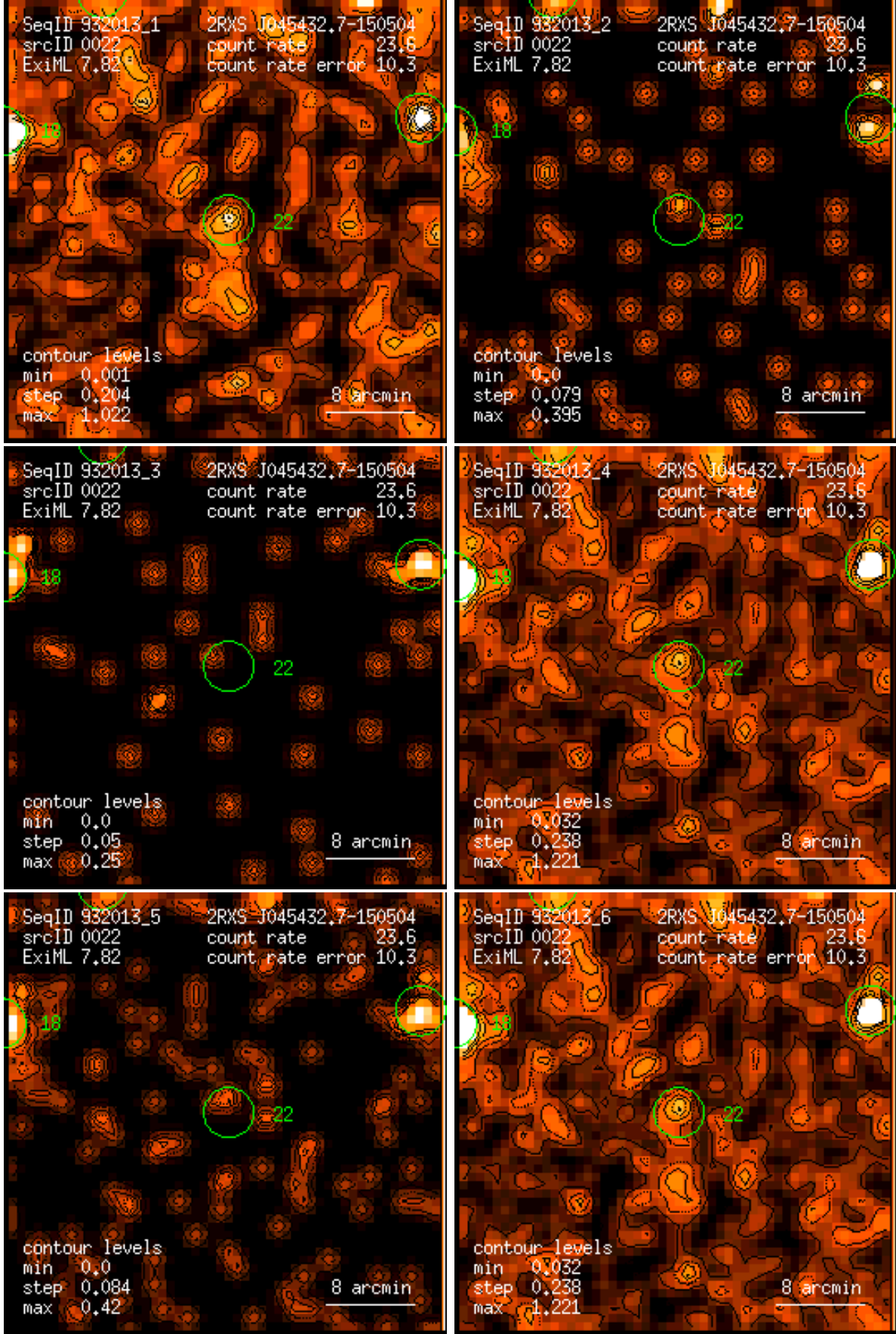
Figure 22: RASS 932013: detection 0022: band rate images, Gaussian filter: (1) PSPC channels 11 – 41, (2) 52 – 90, (3) 91 – 201, (4) 11 – 235, (5) 52 – 201, (6) 11 – 201. Broad band rates in counts/ks. Band rate contour levels in counts/ks/arcmin 2 .
