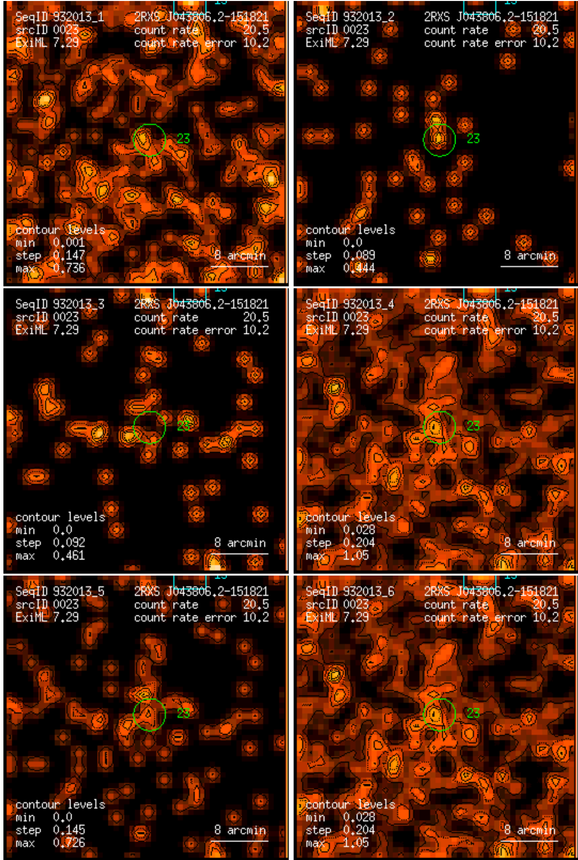
Figure 23: RASS 932013: detection 0023: band rate images, Gaussian filter: (1) PSPC channels 11 – 41, (2) 52 – 90, (3) 91 – 201, (4) 11 – 235, (5) 52 – 201, (6) 11 – 201. Broad band rates in counts/ks. Band rate contour levels in counts/ks/arcmin 2 .
