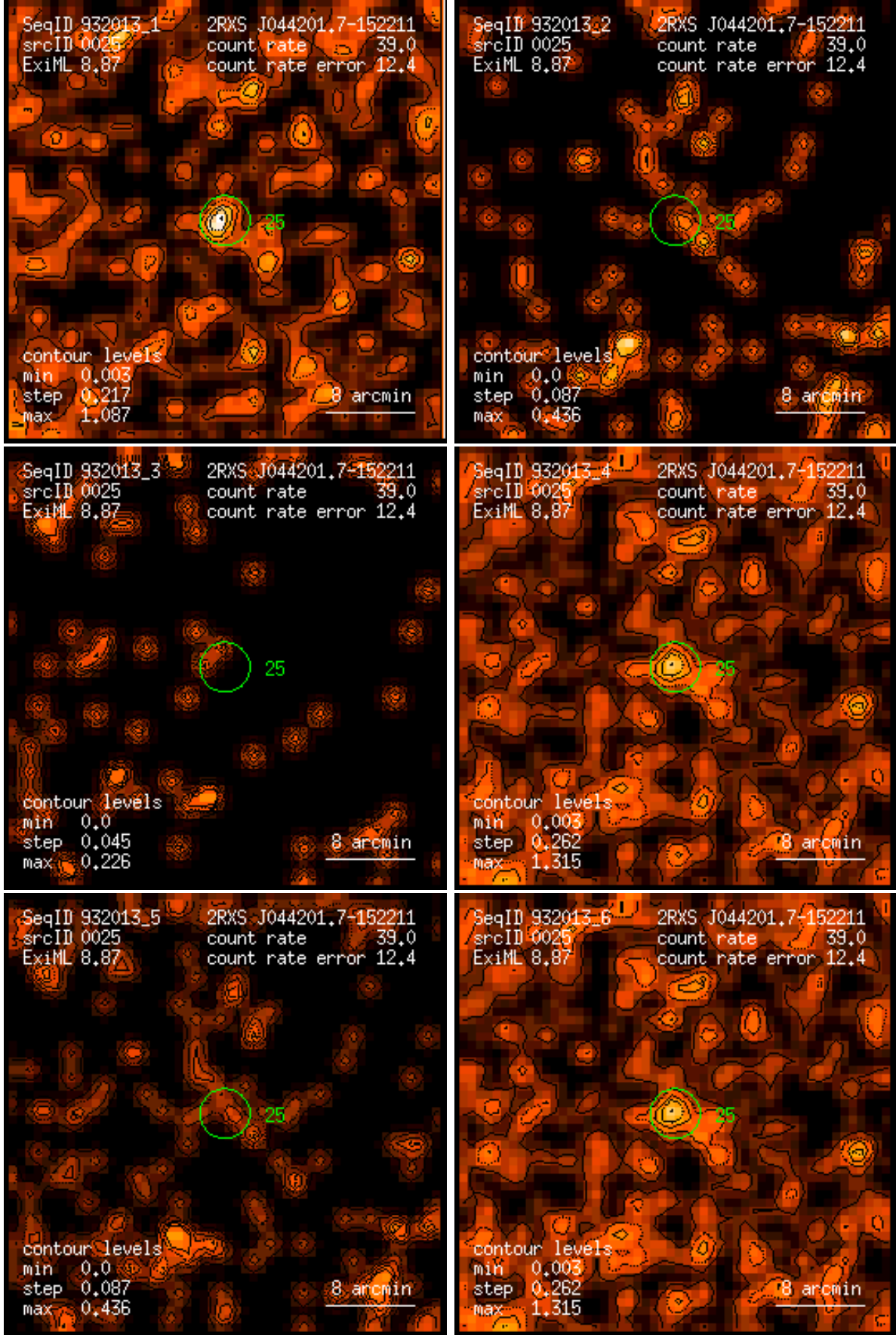
Figure 25: RASS 932013: detection 0025: band rate images, Gaussian filter: (1) PSPC channels 11 – 41, (2) 52 – 90, (3) 91 – 201, (4) 11 – 235, (5) 52 – 201, (6) 11 – 201. Broad band rates in counts/ks. Band rate contour levels in counts/ks/arcmin 2 .
