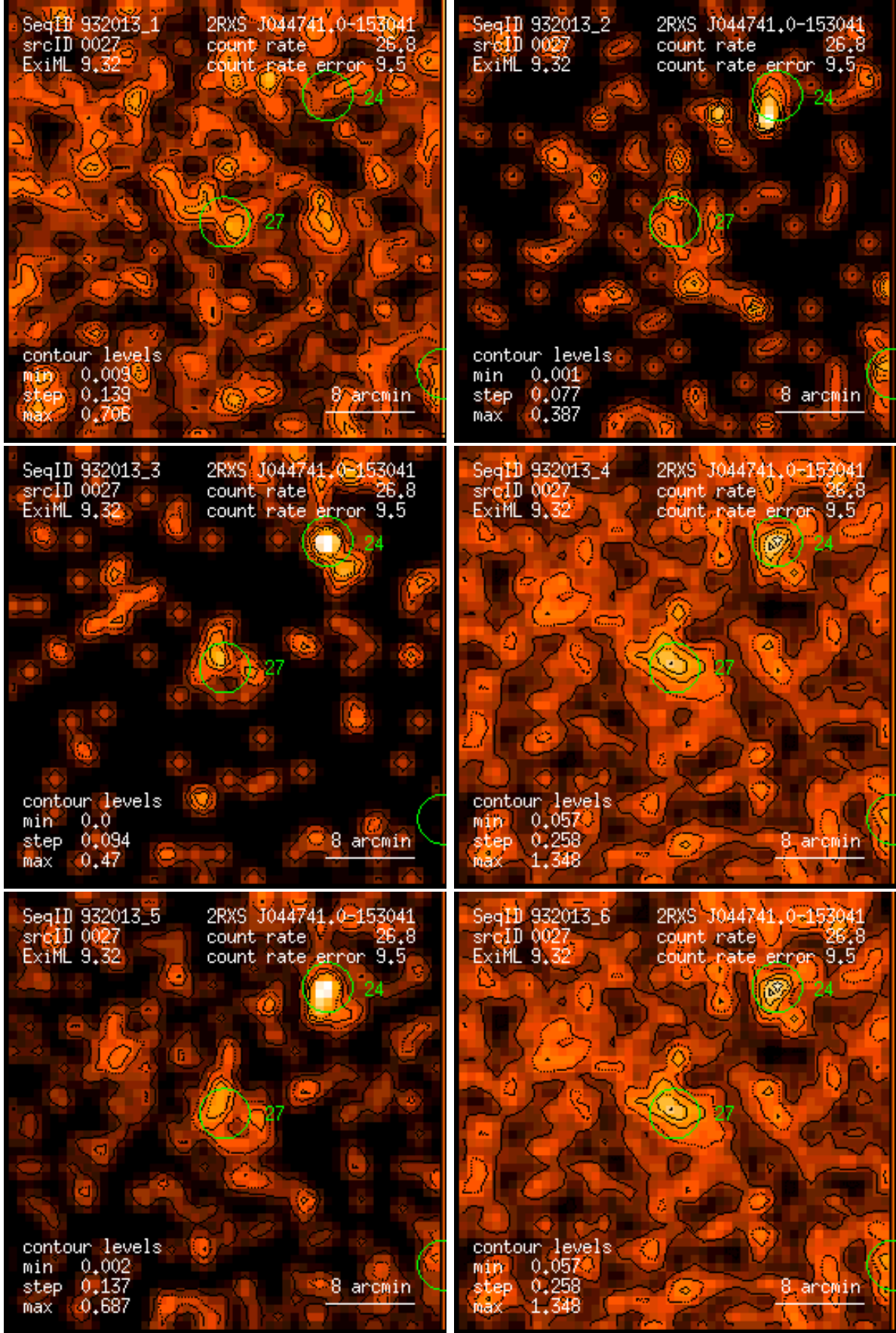
Figure 27: RASS 932013: detection 0027: band rate images, Gaussian filter: (1) PSPC channels 11 – 41, (2) 52 – 90, (3) 91 – 201, (4) 11 – 235, (5) 52 – 201, (6) 11 – 201. Broad band rates in counts/ks. Band rate contour levels in counts/ks/arcmin 2 .
