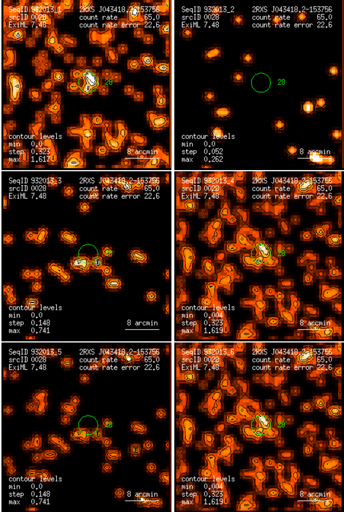
Figure 28: RASS 932013: detection 0028: band rate images, Gaussian filter: (1) PSPC channels 11 – 41, (2) 52 – 90, (3) 91 – 201, (4) 11 – 235, (5) 52 – 201, (6) 11 – 201. Broad band rates in counts/ks. Band rate contour levels in counts/ks/arcmin 2 .
