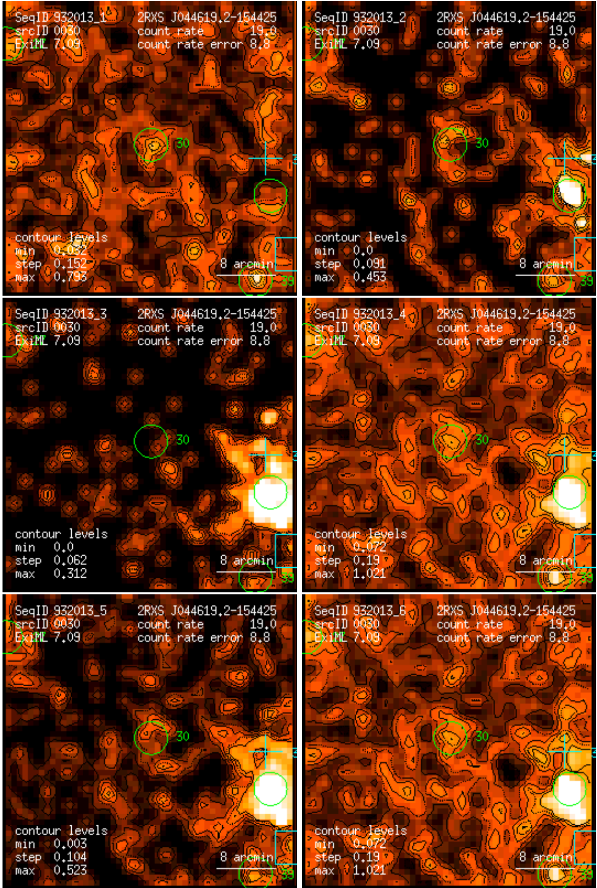
Figure 30: RASS 932013: detection 0030: band rate images, Gaussian filter: (1) PSPC channels 11 – 41, (2) 52 – 90, (3) 91 – 201, (4) 11 – 235, (5) 52 – 201, (6) 11 – 201. Broad band rates in counts/ks. Band rate contour levels in counts/ks/arcmin 2 .
