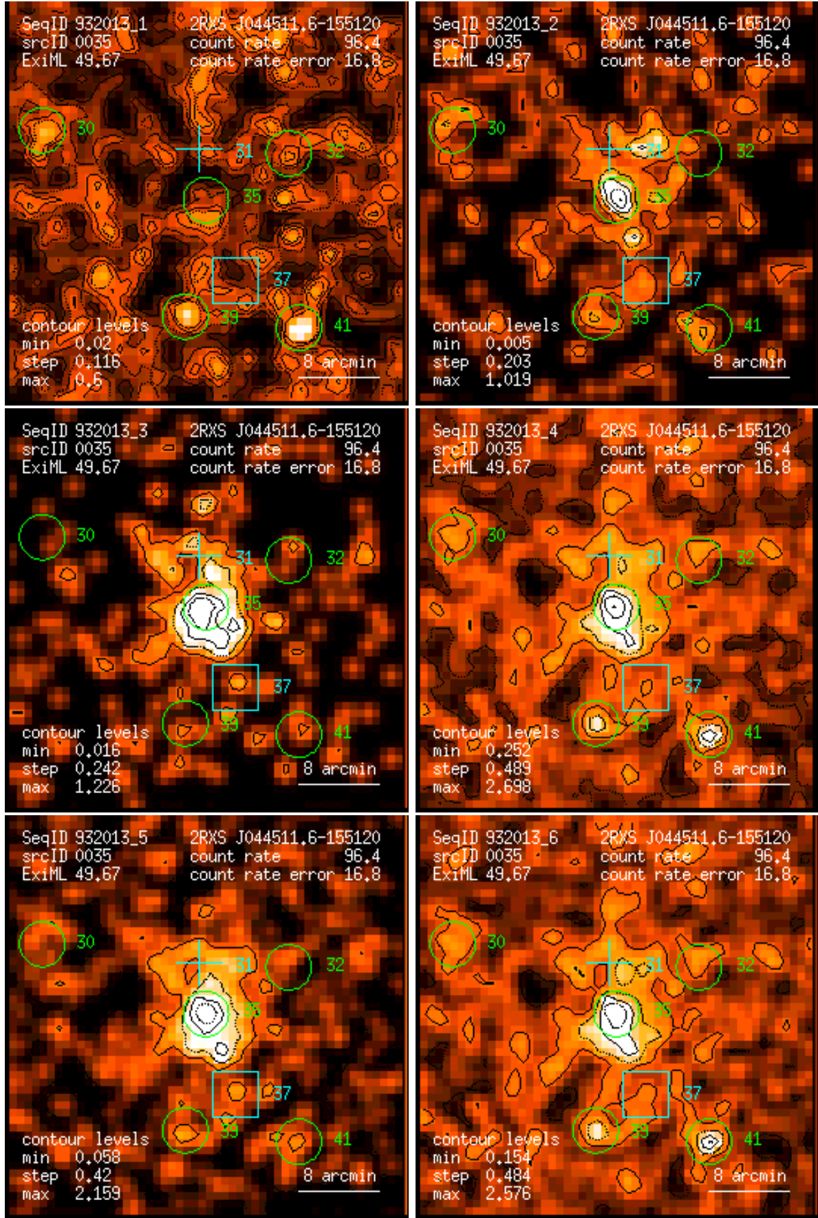
Figure 35: RASS 932013: detection 0035: band rate images, Gaussian filter: (1) PSPC channels 11 – 41, (2) 52 – 90, (3) 91 – 201, (4) 11 – 235, (5) 52 – 201, (6) 11 – 201. Broad band rates in counts/ks. Band rate contour levels in counts/ks/arcmin 2 .
