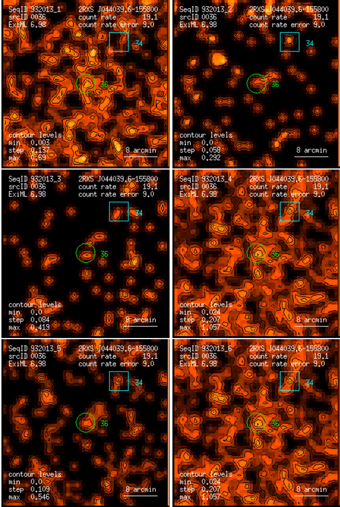
Figure 36: RASS 932013: detection 0036: band rate images, Gaussian filter: (1) PSPC channels 11 – 41, (2) 52 – 90, (3) 91 – 201, (4) 11 – 235, (5) 52 – 201, (6) 11 – 201. Broad band rates in counts/ks. Band rate contour levels in counts/ks/arcmin 2 .
