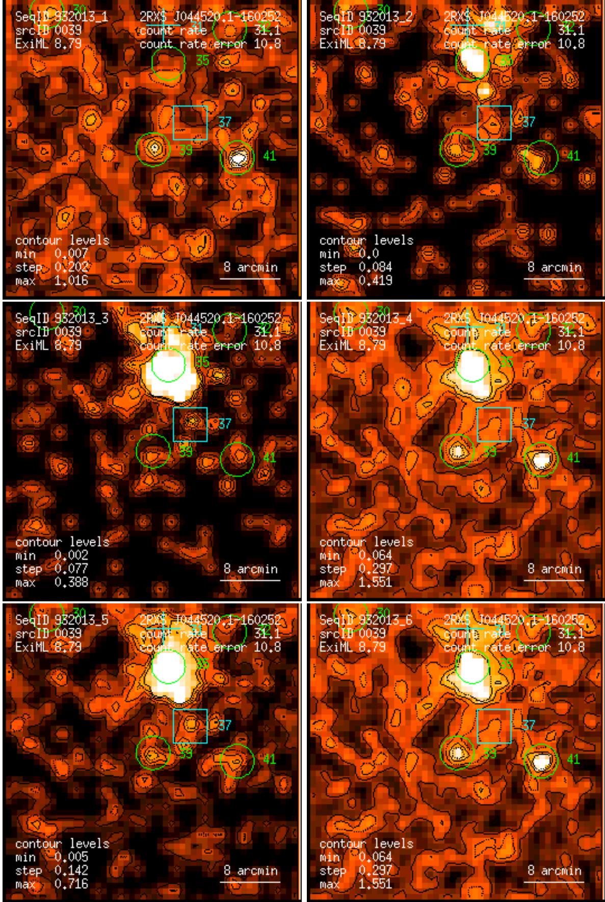
Figure 39: RASS 932013: detection 0039: band rate images, Gaussian filter: (1) PSPC channels 11 – 41, (2) 52 – 90, (3) 91 – 201, (4) 11 – 235, (5) 52 – 201, (6) 11 – 201. Broad band rates in counts/ks. Band rate contour levels in counts/ks/arcmin 2 .
