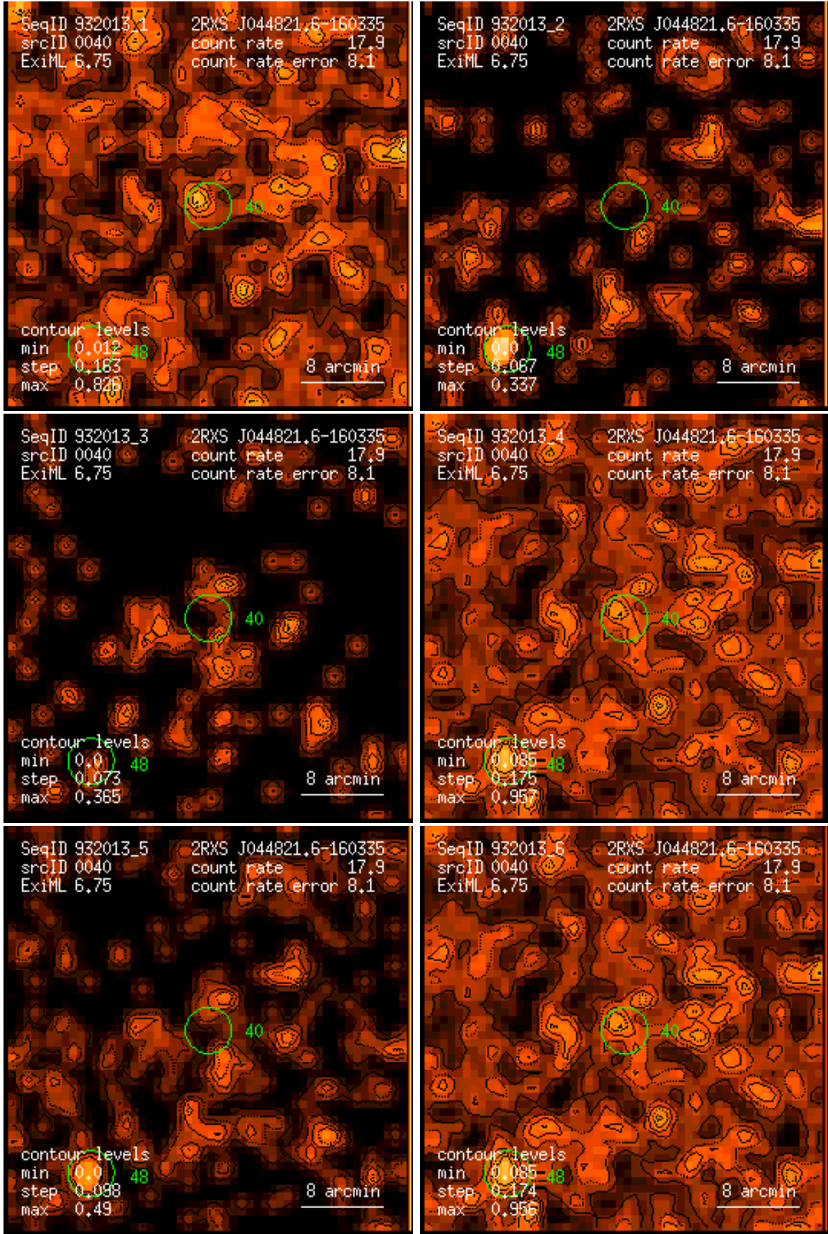
Figure 40: RASS 932013: detection 0040: band rate images, Gaussian filter: (1) PSPC channels 11 – 41, (2) 52 – 90, (3) 91 – 201, (4) 11 – 235, (5) 52 – 201, (6) 11 – 201. Broad band rates in counts/ks. Band rate contour levels in counts/ks/arcmin 2 .
