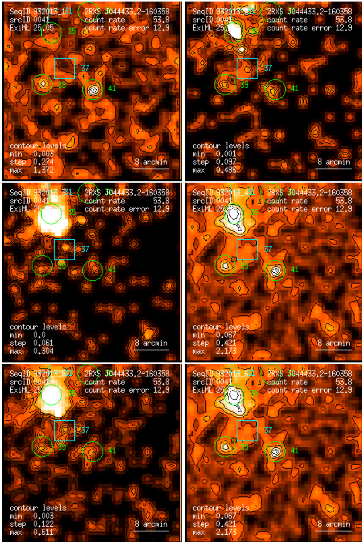
Figure 41: RASS 932013: detection 0041: band rate images, Gaussian filter: (1) PSPC channels 11 – 41, (2) 52 – 90, (3) 91 – 201, (4) 11 – 235, (5) 52 – 201, (6) 11 – 201. Broad band rates in counts/ks. Band rate contour levels in counts/ks/arcmin 2 .
