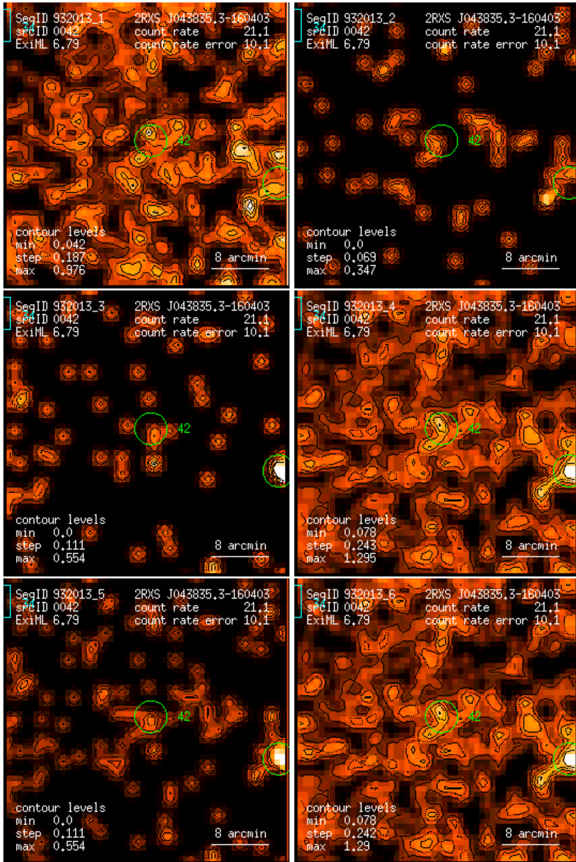
Figure 42: RASS 932013: detection 0042: band rate images, Gaussian filter: (1) PSPC channels 11 – 41, (2) 52 – 90, (3) 91 – 201, (4) 11 – 235, (5) 52 – 201, (6) 11 – 201. Broad band rates in counts/ks. Band rate contour levels in counts/ks/arcmin 2 .
