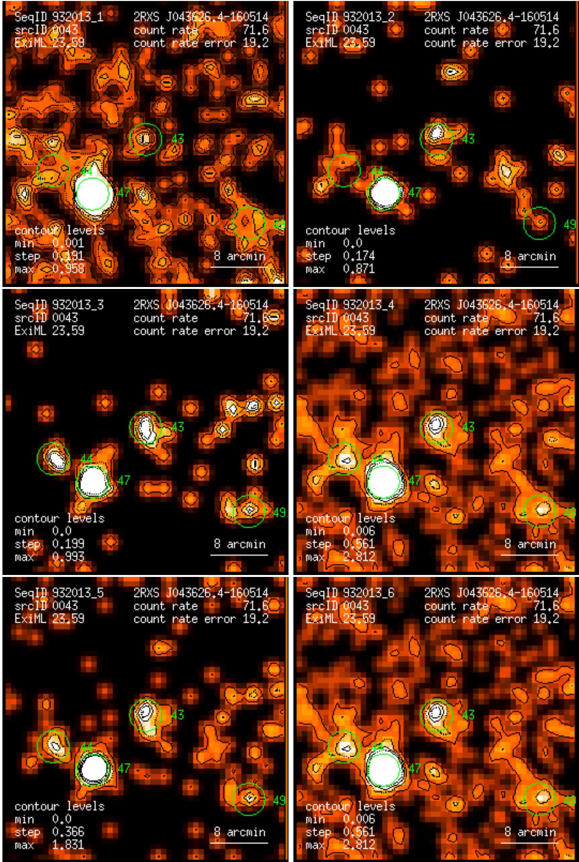
Figure 43: RASS 932013: detection 0043: band rate images, Gaussian filter: (1) PSPC channels 11 – 41, (2) 52 – 90, (3) 91 – 201, (4) 11 – 235, (5) 52 – 201, (6) 11 – 201. Broad band rates in counts/ks. Band rate contour levels in counts/ks/arcmin 2 .
