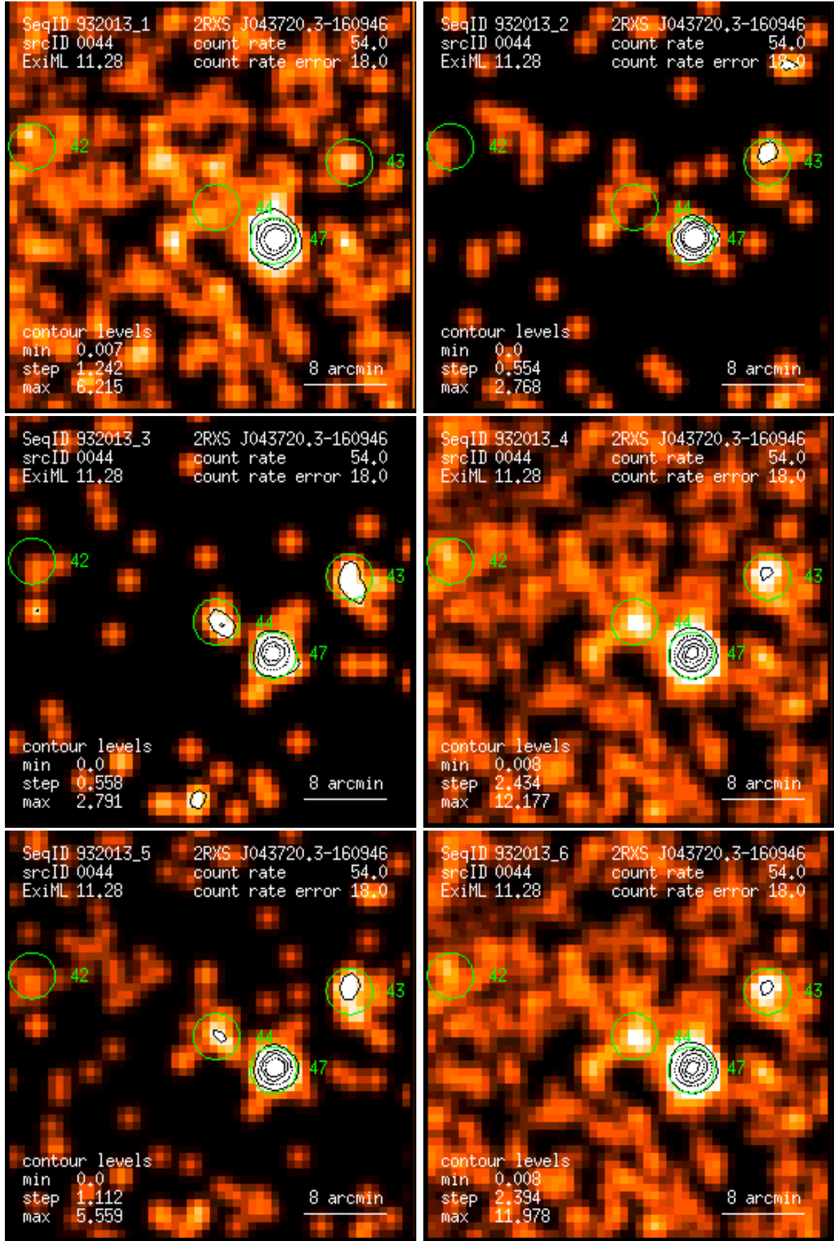
Figure 44: RASS 932013: detection 0044: band rate images, Gaussian filter: (1) PSPC channels 11 – 41, (2) 52 – 90, (3) 91 – 201, (4) 11 – 235, (5) 52 – 201, (6) 11 – 201. Broad band rates in counts/ks. Band rate contour levels in counts/ks/arcmin 2 .
