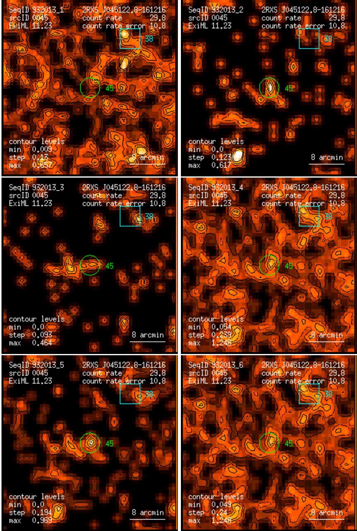
Figure 45: RASS 932013: detection 0045: band rate images, Gaussian filter: (1) PSPC channels 11 – 41, (2) 52 – 90, (3) 91 – 201, (4) 11 – 235, (5) 52 – 201, (6) 11 – 201. Broad band rates in counts/ks. Band rate contour levels in counts/ks/arcmin 2 .
