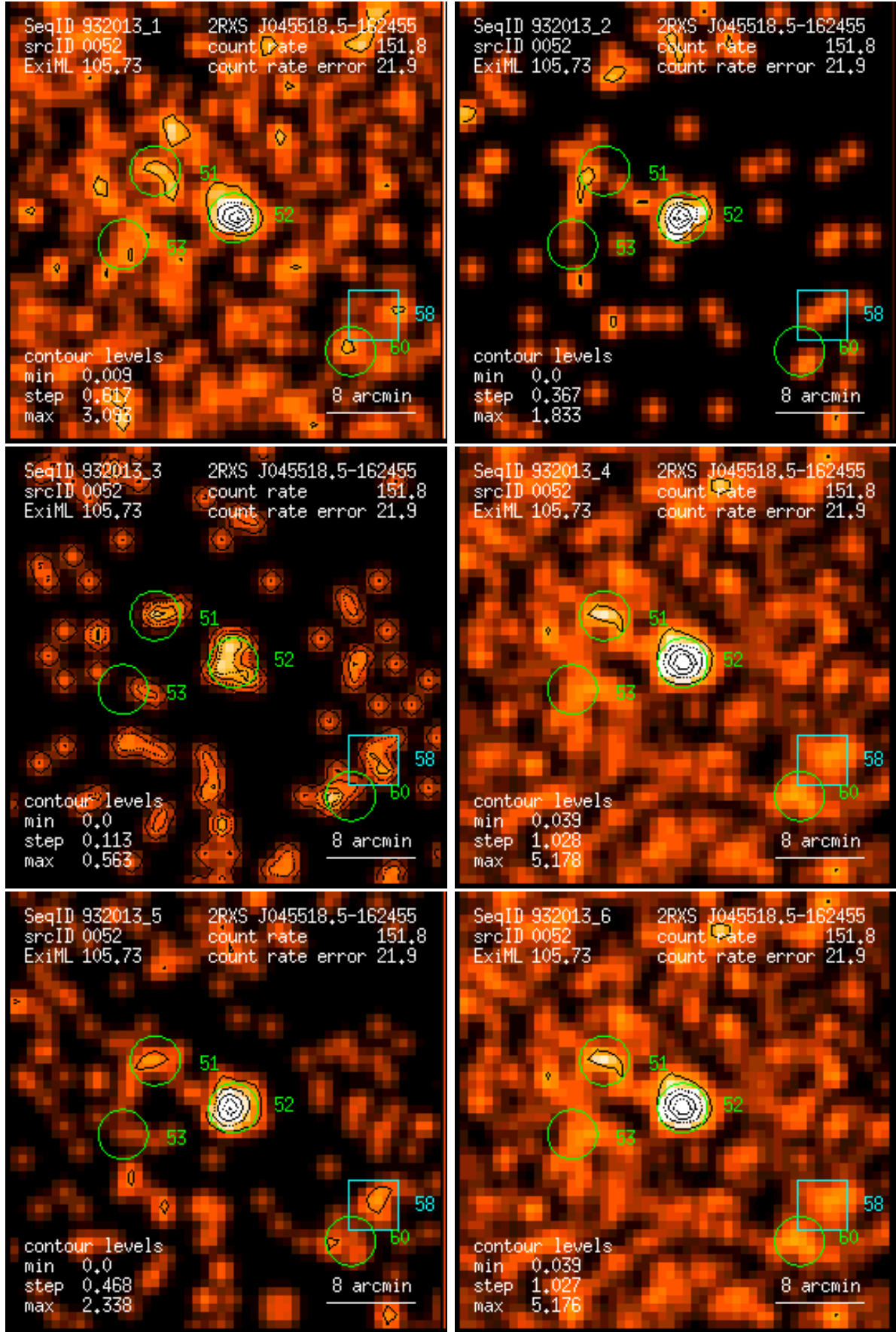
Figure 52: RASS 932013: detection 0052: band rate images, Gaussian filter: (1) PSPC channels 11 – 41, (2) 52 – 90, (3) 91 – 201, (4) 11 – 235, (5) 52 – 201, (6) 11 – 201. Broad band rates in counts/ks. Band rate contour levels in counts/ks/arcmin 2 .
