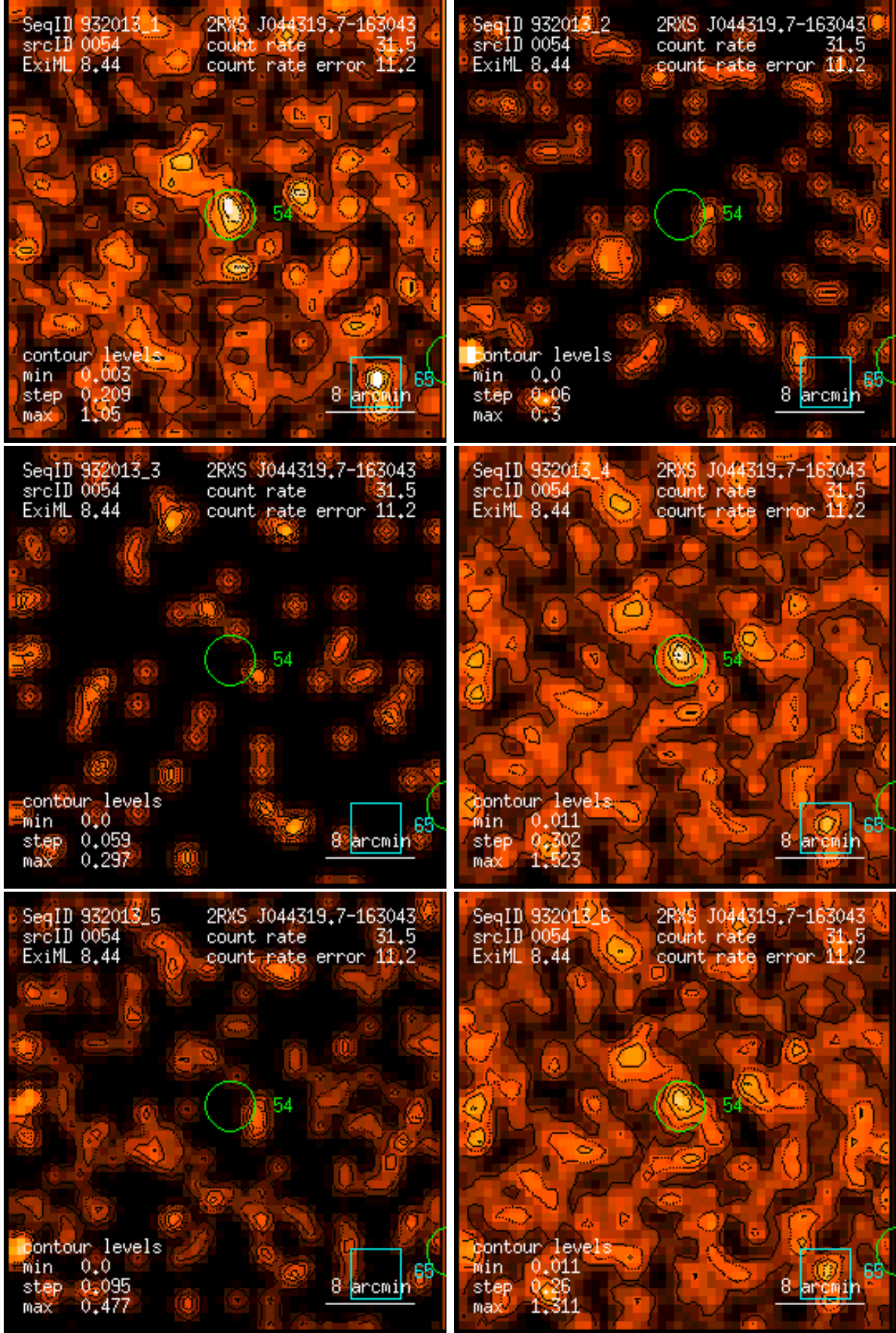
Figure 54: RASS 932013: detection 0054: band rate images, Gaussian filter: (1) PSPC channels 11 – 41, (2) 52 – 90, (3) 91 – 201, (4) 11 – 235, (5) 52 – 201, (6) 11 – 201. Broad band rates in counts/ks. Band rate contour levels in counts/ks/arcmin 2 .
