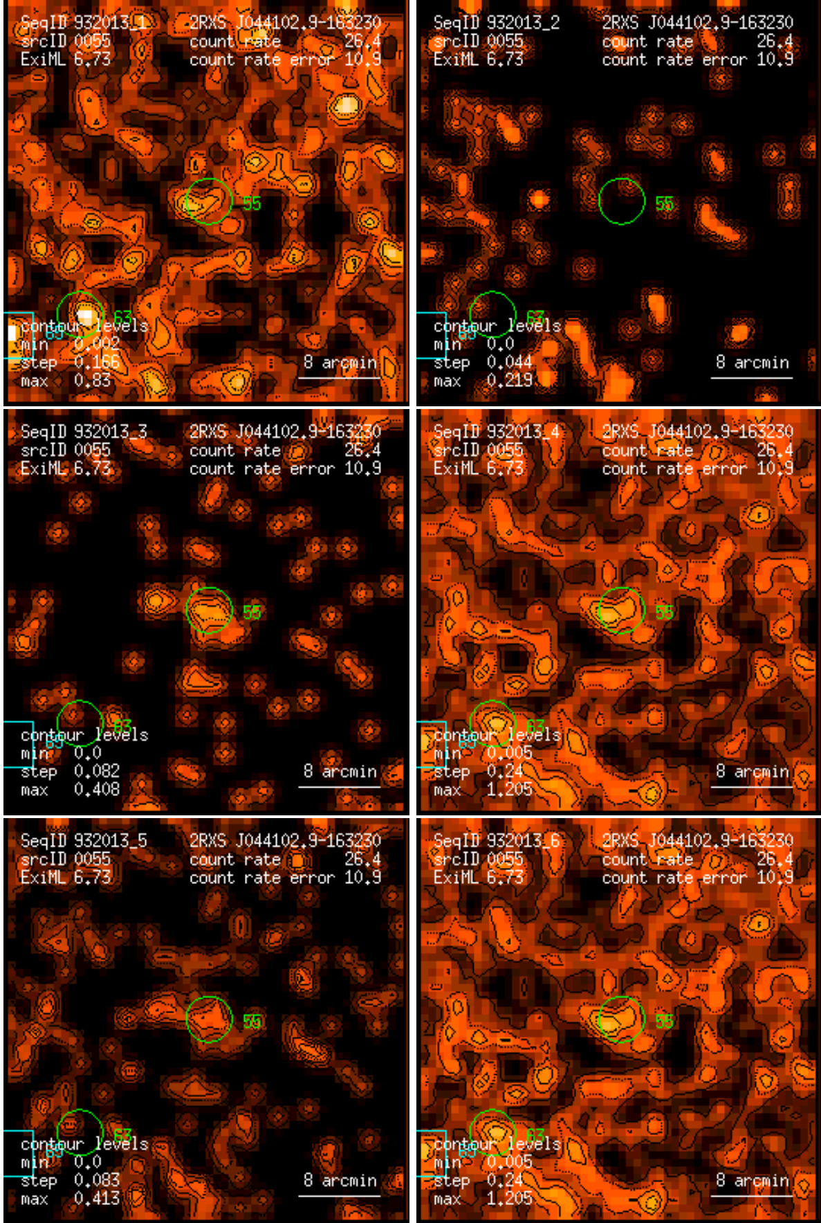
Figure 55: RASS 932013: detection 0055: band rate images, Gaussian filter: (1) PSPC channels 11 – 41, (2) 52 – 90, (3) 91 – 201, (4) 11 – 235, (5) 52 – 201, (6) 11 – 201. Broad band rates in counts/ks. Band rate contour levels in counts/ks/arcmin 2 .
