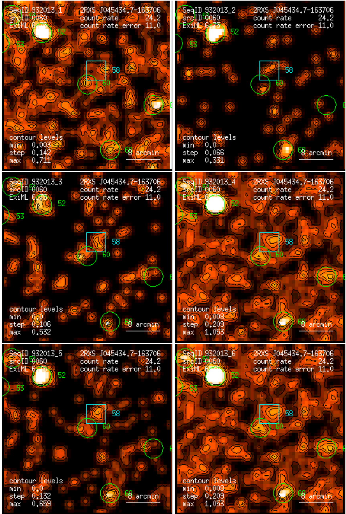
Figure 60: RASS 932013: detection 0060: band rate images, Gaussian filter: (1) PSPC channels 11 – 41, (2) 52 – 90, (3) 91 – 201, (4) 11 – 235, (5) 52 – 201, (6) 11 – 201. Broad band rates in counts/ks. Band rate contour levels in counts/ks/arcmin 2 .
