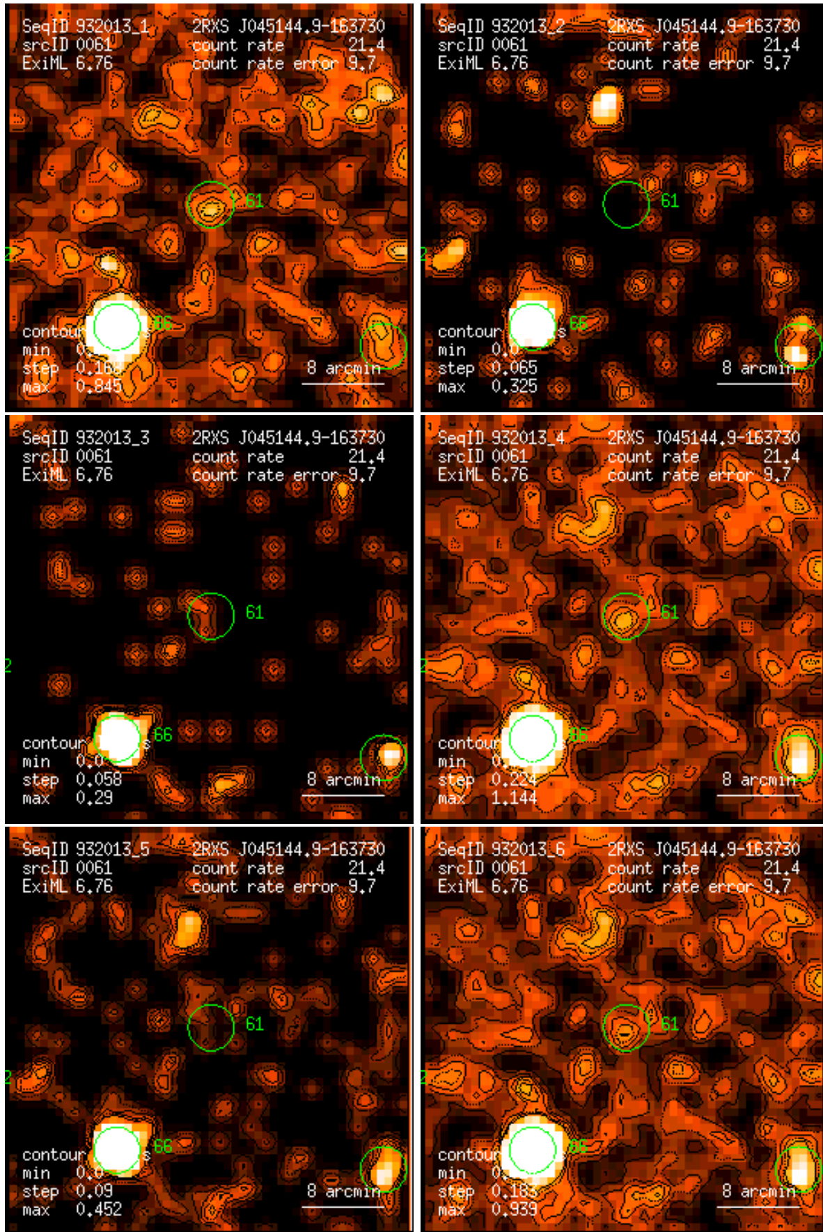
Figure 61: RASS 932013: detection 0061: band rate images, Gaussian filter: (1) PSPC channels 11 – 41, (2) 52 – 90, (3) 91 – 201, (4) 11 – 235, (5) 52 – 201, (6) 11 – 201. Broad band rates in counts/ks. Band rate contour levels in counts/ks/arcmin 2 .
