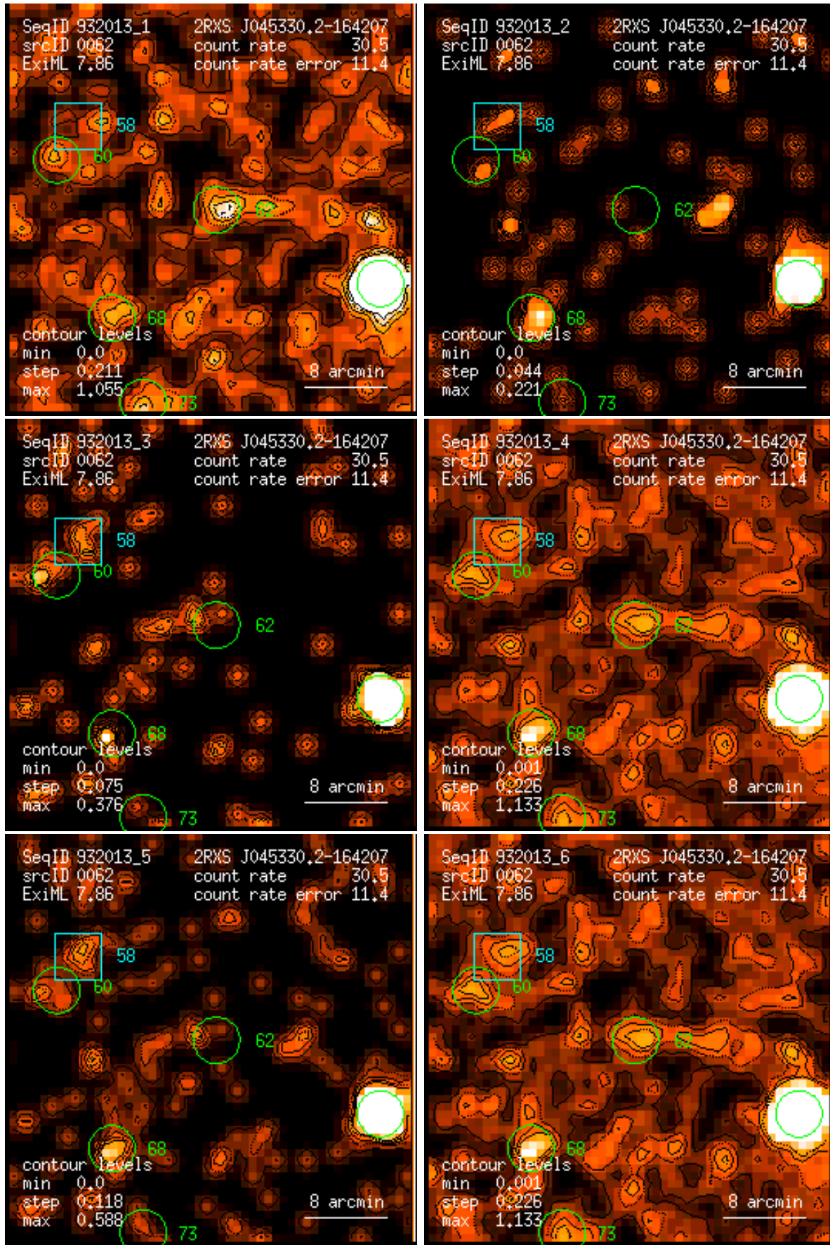
Figure 62: RASS 932013: detection 0062: band rate images, Gaussian filter: (1) PSPC channels 11 – 41, (2) 52 – 90, (3) 91 – 201, (4) 11 – 235, (5) 52 – 201, (6) 11 – 201. Broad band rates in counts/ks. Band rate contour levels in counts/ks/arcmin 2 .
