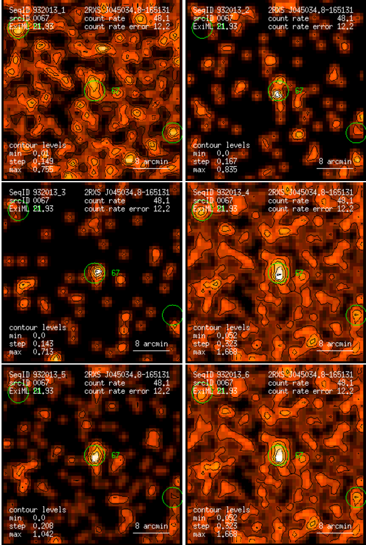
Figure 67: RASS 932013: detection 0067: band rate images, Gaussian filter: (1) PSPC channels 11 – 41, (2) 52 – 90, (3) 91 – 201, (4) 11 – 235, (5) 52 – 201, (6) 11 – 201. Broad band rates in counts/ks. Band rate contour levels in counts/ks/arcmin 2 .
