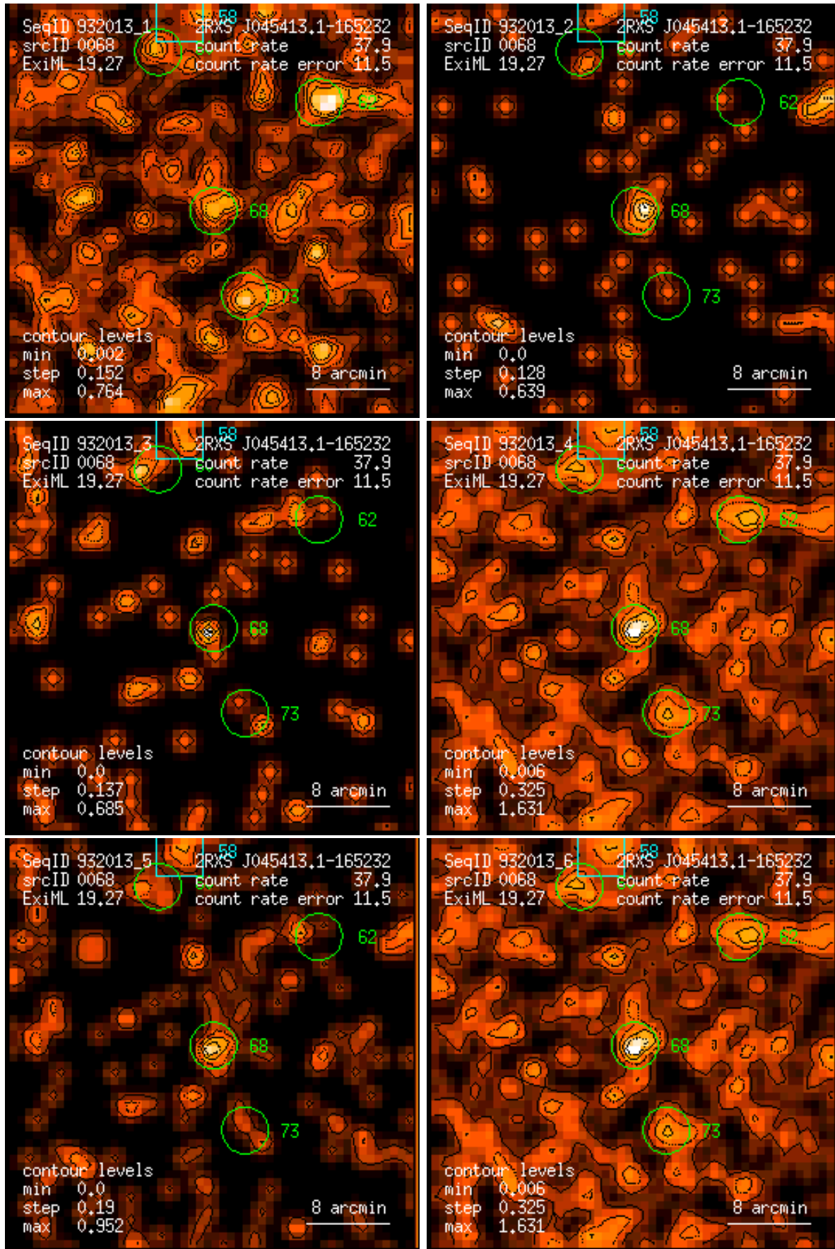
Figure 68: RASS 932013: detection 0068: band rate images, Gaussian filter: (1) PSPC channels 11 – 41, (2) 52 – 90, (3) 91 – 201, (4) 11 – 235, (5) 52 – 201, (6) 11 – 201. Broad band rates in counts/ks. Band rate contour levels in counts/ks/arcmin 2 .
