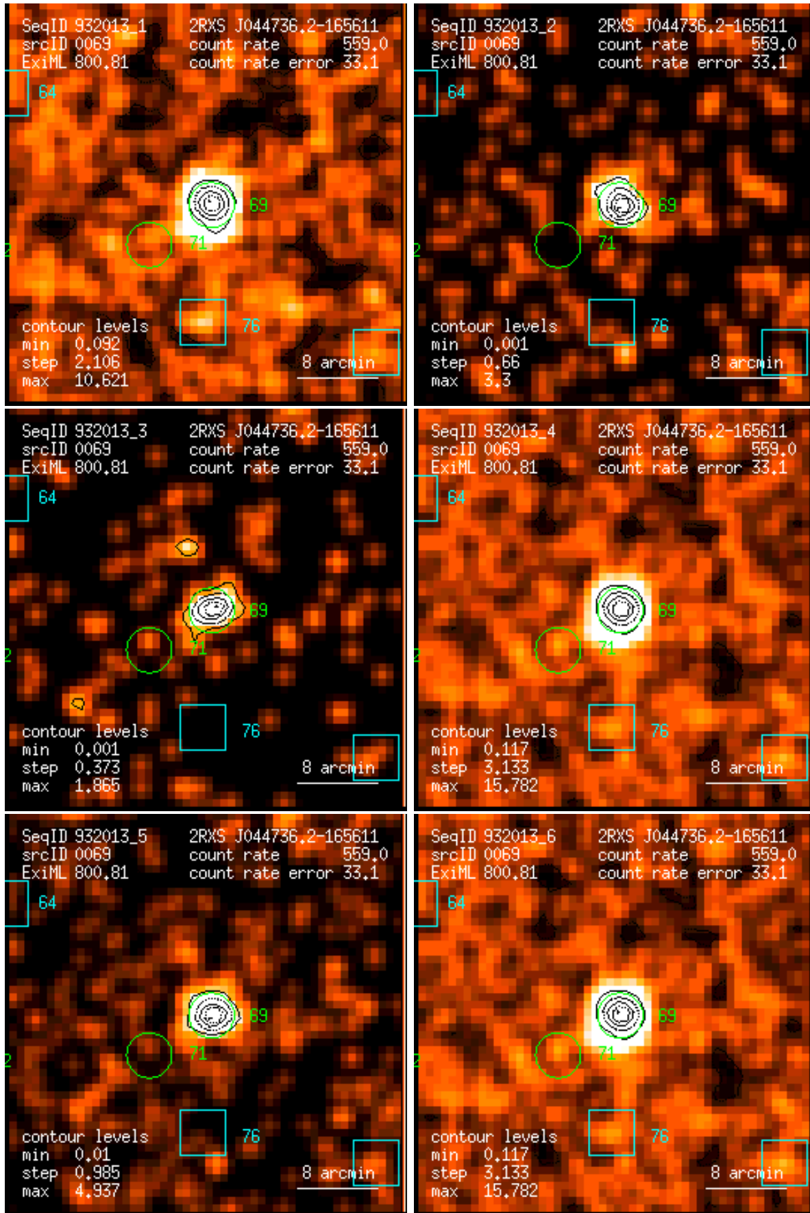
Figure 69: RASS 932013: detection 0069: band rate images, Gaussian filter: (1) PSPC channels 11 – 41, (2) 52 – 90, (3) 91 – 201, (4) 11 – 235, (5) 52 – 201, (6) 11 – 201. Broad band rates in counts/ks. Band rate contour levels in counts/ks/arcmin 2 .
