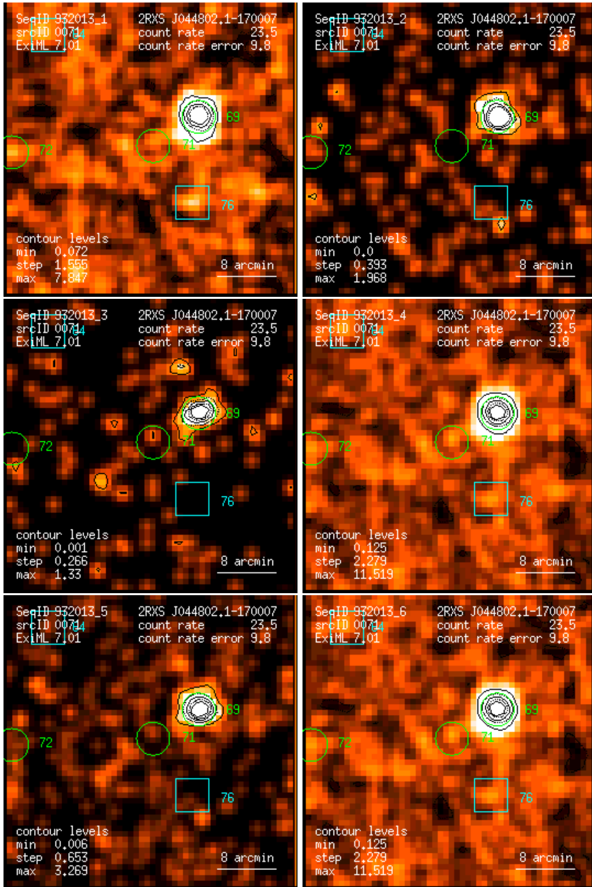
Figure 71: RASS 932013: detection 0071: band rate images, Gaussian filter: (1) PSPC channels 11 – 41, (2) 52 – 90, (3) 91 – 201, (4) 11 – 235, (5) 52 – 201, (6) 11 – 201. Broad band rates in counts/ks. Band rate contour levels in counts/ks/arcmin 2 .
