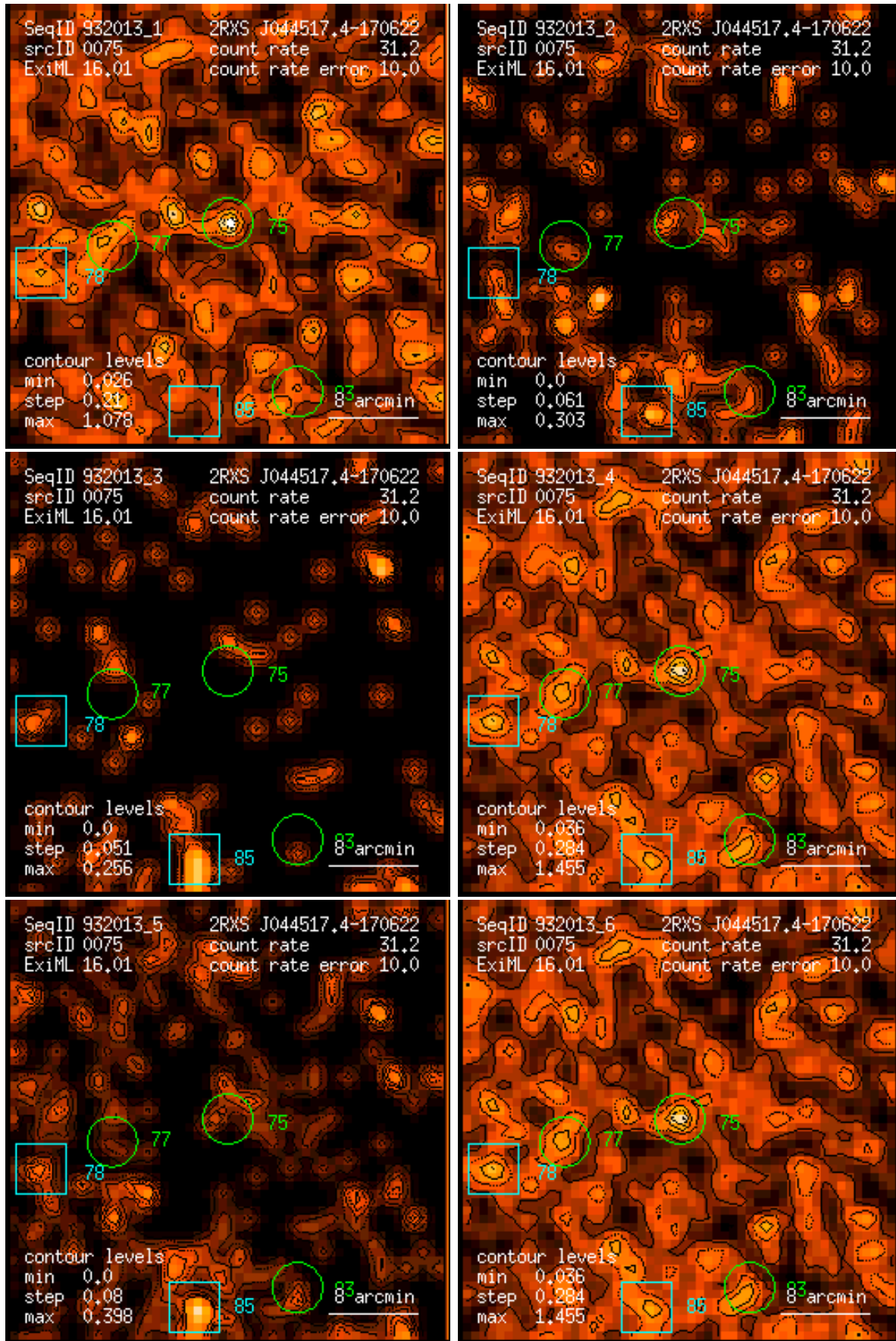
Figure 75: RASS 932013: detection 0075: band rate images, Gaussian filter: (1) PSPC channels 11 – 41, (2) 52 – 90, (3) 91 – 201, (4) 11 – 235, (5) 52 – 201, (6) 11 – 201. Broad band rates in counts/ks. Band rate contour levels in counts/ks/arcmin 2 .
