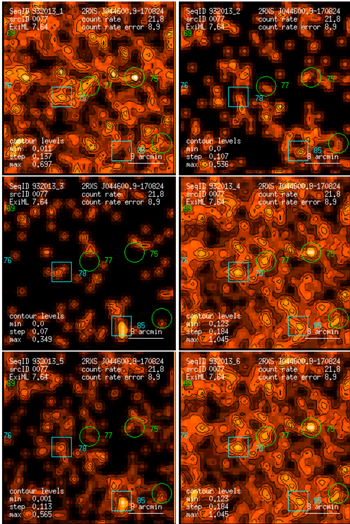
Figure 77: RASS 932013: detection 0077: band rate images, Gaussian filter: (1) PSPC channels 11 – 41, (2) 52 – 90, (3) 91 – 201, (4) 11 – 235, (5) 52 – 201, (6) 11 – 201. Broad band rates in counts/ks. Band rate contour levels in counts/ks/arcmin 2 .
