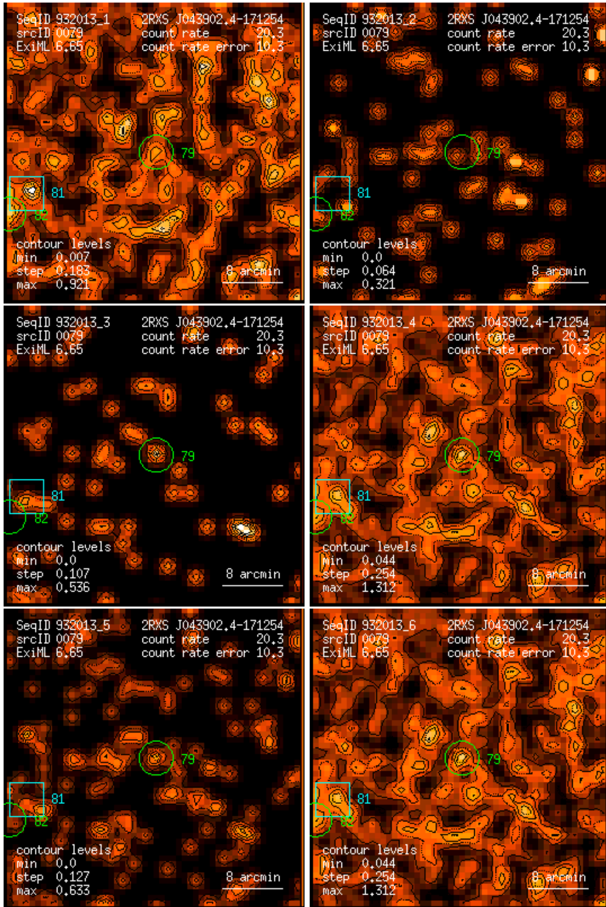
Figure 79: RASS 932013: detection 0079: band rate images, Gaussian filter: (1) PSPC channels 11 – 41, (2) 52 – 90, (3) 91 – 201, (4) 11 – 235, (5) 52 – 201, (6) 11 – 201. Broad band rates in counts/ks. Band rate contour levels in counts/ks/arcmin 2 .
