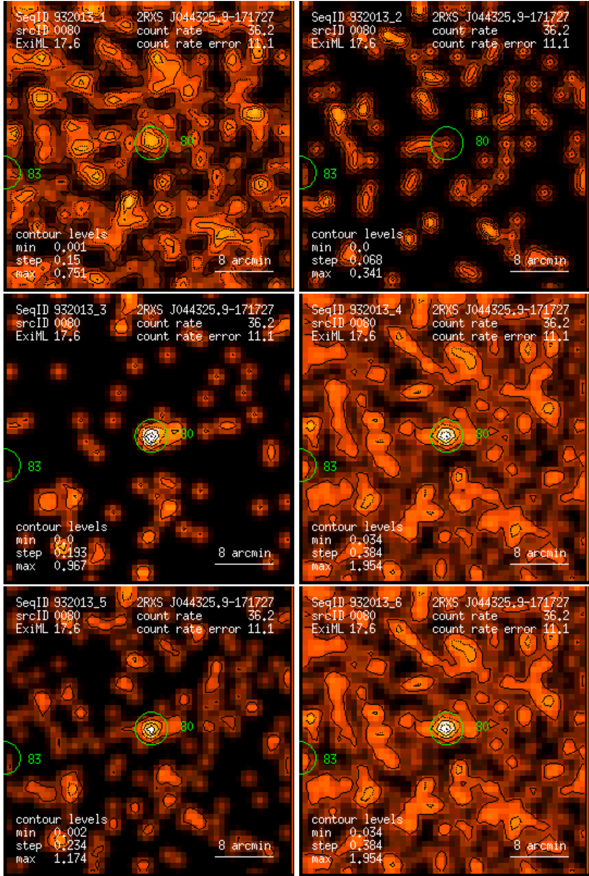
Figure 80: RASS 932013: detection 0080: band rate images, Gaussian filter: (1) PSPC channels 11 – 41, (2) 52 – 90, (3) 91 – 201, (4) 11 – 235, (5) 52 – 201, (6) 11 – 201. Broad band rates in counts/ks. Band rate contour levels in counts/ks/arcmin 2 .
