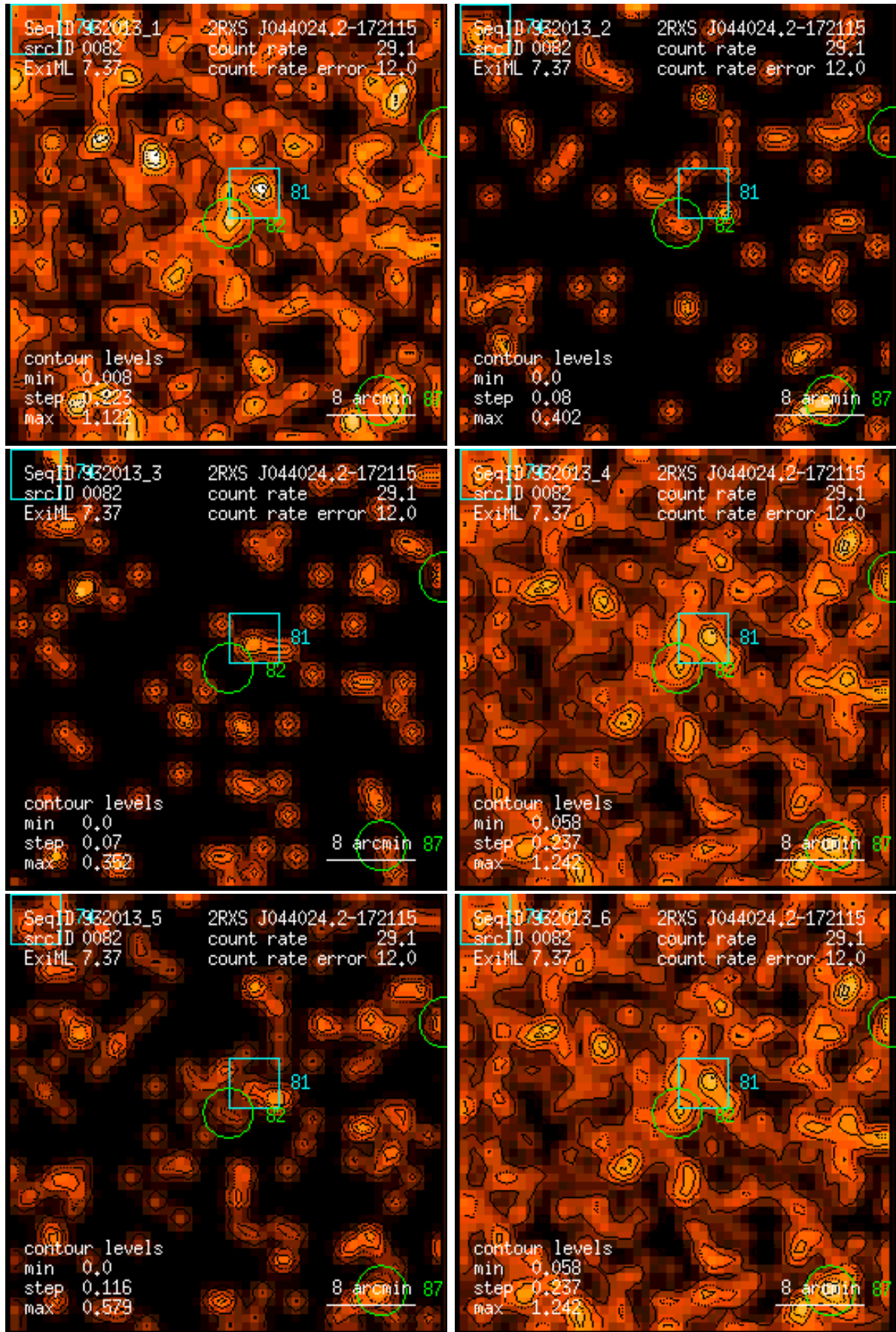
Figure 82: RASS 932013: detection 0082: band rate images, Gaussian filter: (1) PSPC channels 11 – 41, (2) 52 – 90, (3) 91 – 201, (4) 11 – 235, (5) 52 – 201, (6) 11 – 201. Broad band rates in counts/ks. Band rate contour levels in counts/ks/arcmin 2 .
