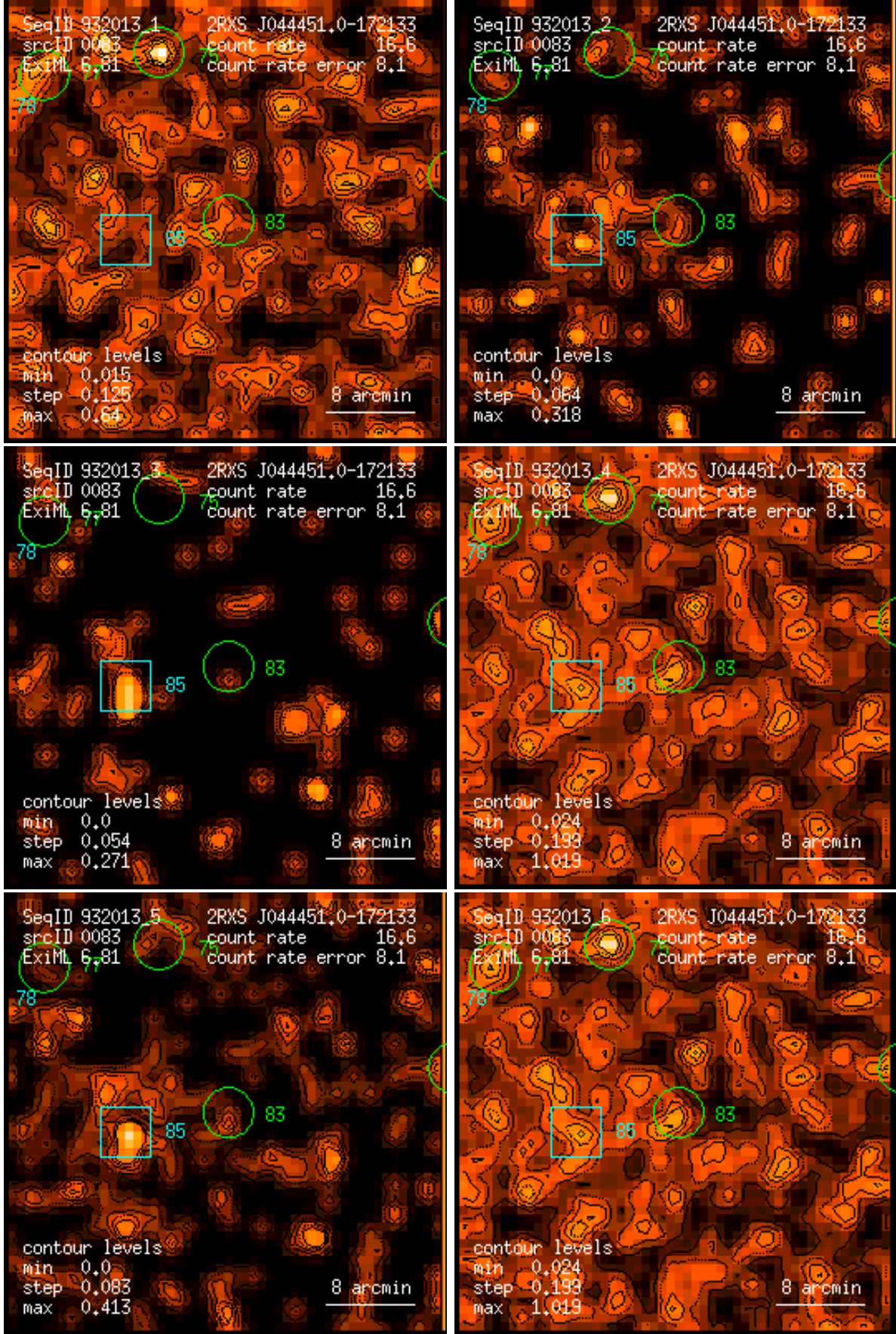
Figure 83: RASS 932013: detection 0083: band rate images, Gaussian filter: (1) PSPC channels 11 – 41, (2) 52 – 90, (3) 91 – 201, (4) 11 – 235, (5) 52 – 201, (6) 11 – 201. Broad band rates in counts/ks. Band rate contour levels in counts/ks/arcmin 2 .
