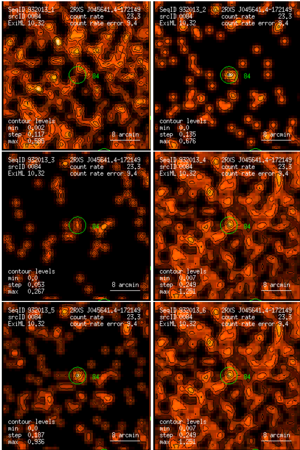
Figure 84: RASS 932013: detection 0084: band rate images, Gaussian filter: (1) PSPC channels 11 – 41, (2) 52 – 90, (3) 91 – 201, (4) 11 – 235, (5) 52 – 201, (6) 11 – 201. Broad band rates in counts/ks. Band rate contour levels in counts/ks/arcmin 2 .
