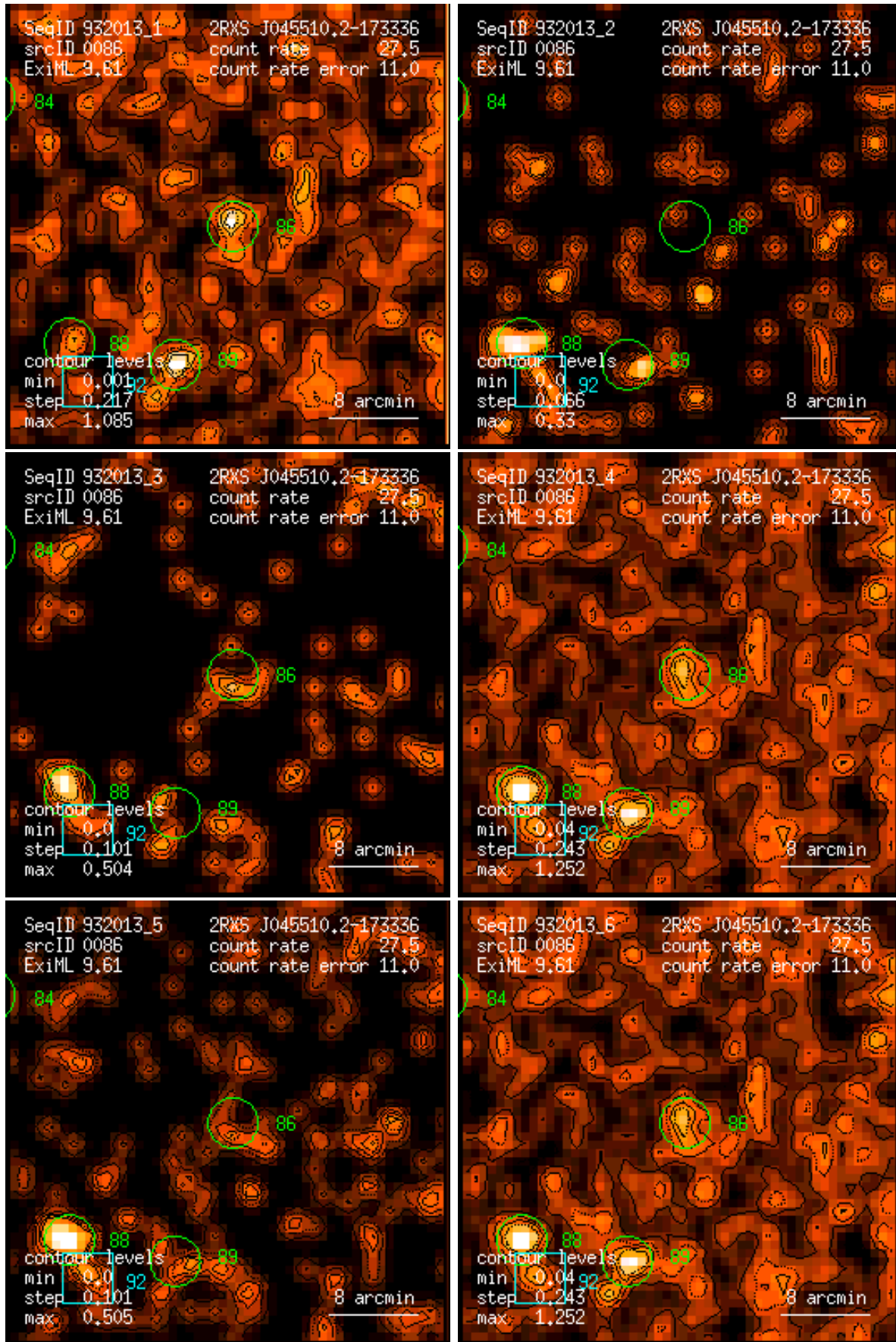
Figure 86: RASS 932013: detection 0086: band rate images, Gaussian filter: (1) PSPC channels 11 – 41, (2) 52 – 90, (3) 91 – 201, (4) 11 – 235, (5) 52 – 201, (6) 11 – 201. Broad band rates in counts/ks. Band rate contour levels in counts/ks/arcmin 2 .
