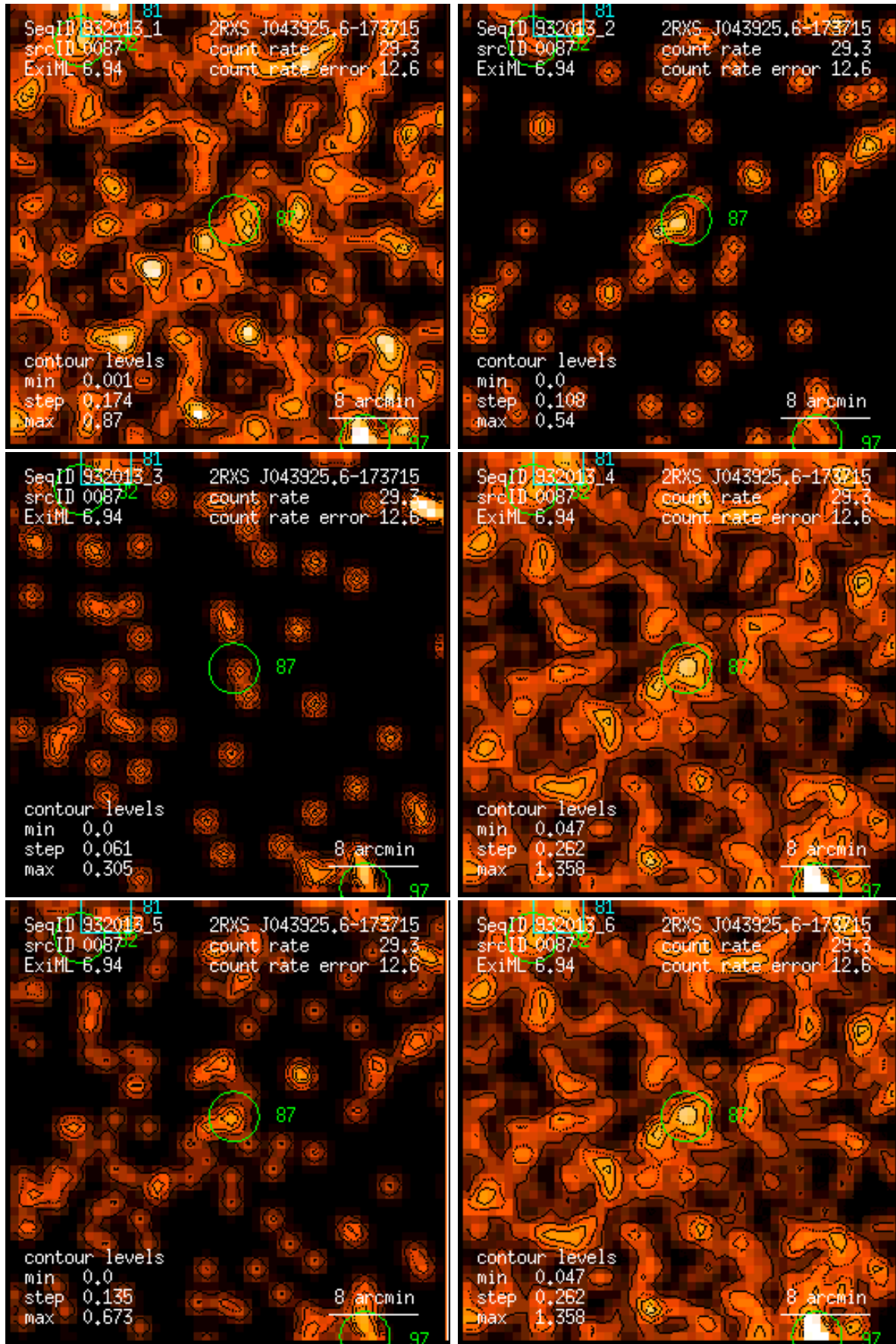
Figure 87: RASS 932013: detection 0087: band rate images, Gaussian filter: (1) PSPC channels 11 – 41, (2) 52 – 90, (3) 91 – 201, (4) 11 – 235, (5) 52 – 201, (6) 11 – 201. Broad band rates in counts/ks. Band rate contour levels in counts/ks/arcmin 2 .
