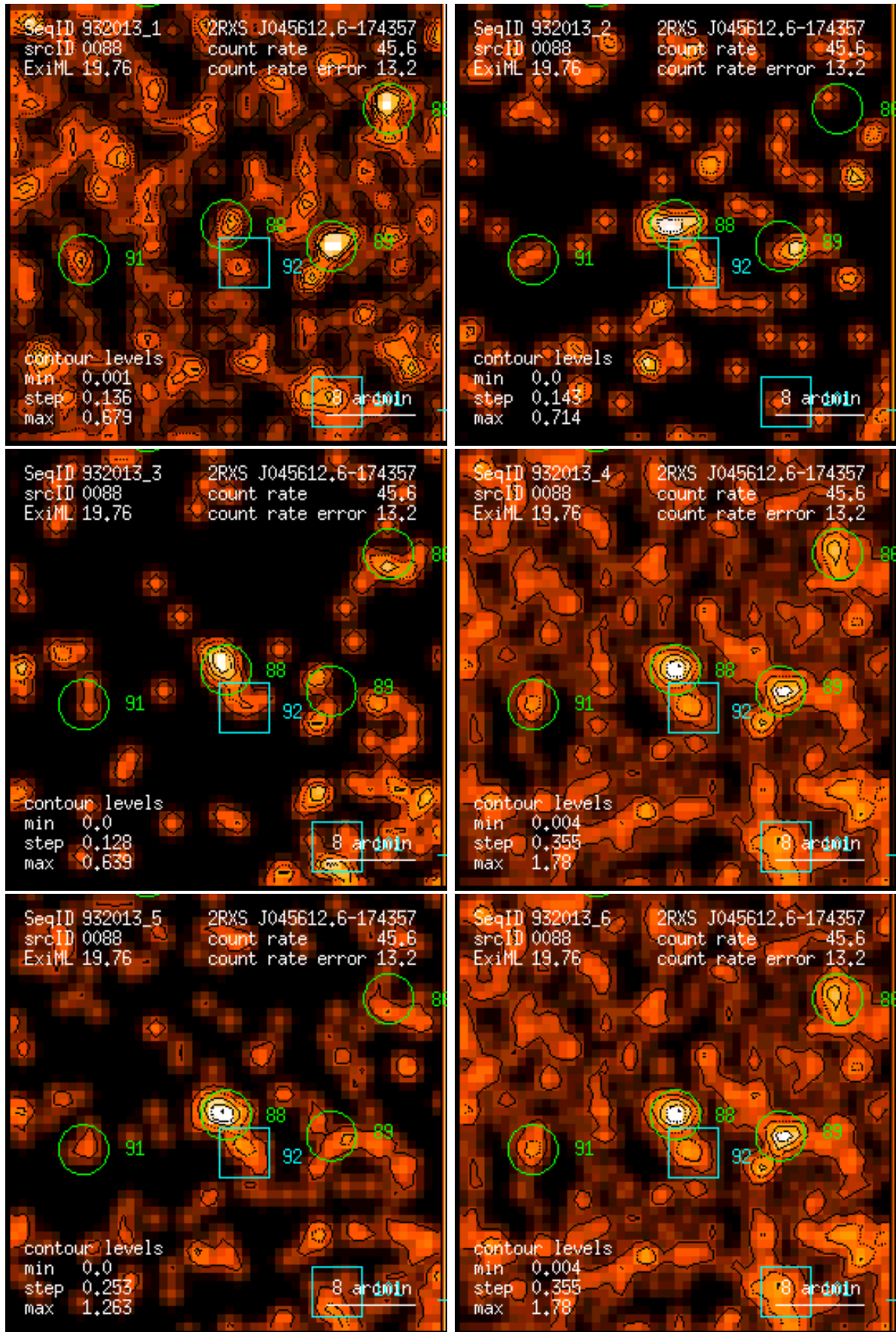
Figure 88: RASS 932013: detection 0088: band rate images, Gaussian filter: (1) PSPC channels 11 – 41, (2) 52 – 90, (3) 91 – 201, (4) 11 – 235, (5) 52 – 201, (6) 11 – 201. Broad band rates in counts/ks. Band rate contour levels in counts/ks/arcmin 2 .
