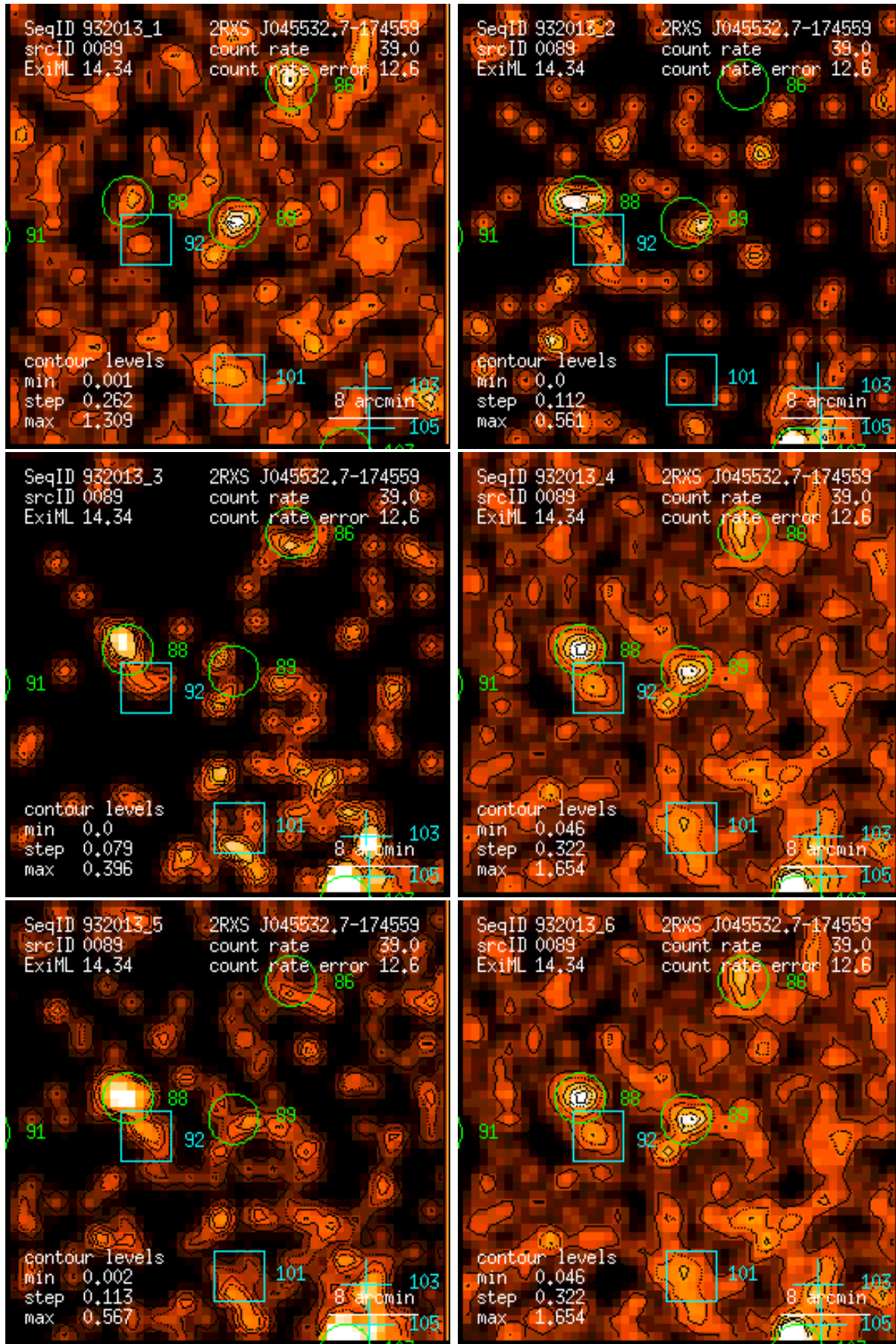
Figure 89: RASS 932013: detection 0089: band rate images, Gaussian filter: (1) PSPC channels 11 – 41, (2) 52 – 90, (3) 91 – 201, (4) 11 – 235, (5) 52 – 201, (6) 11 – 201. Broad band rates in counts/ks. Band rate contour levels in counts/ks/arcmin 2 .
