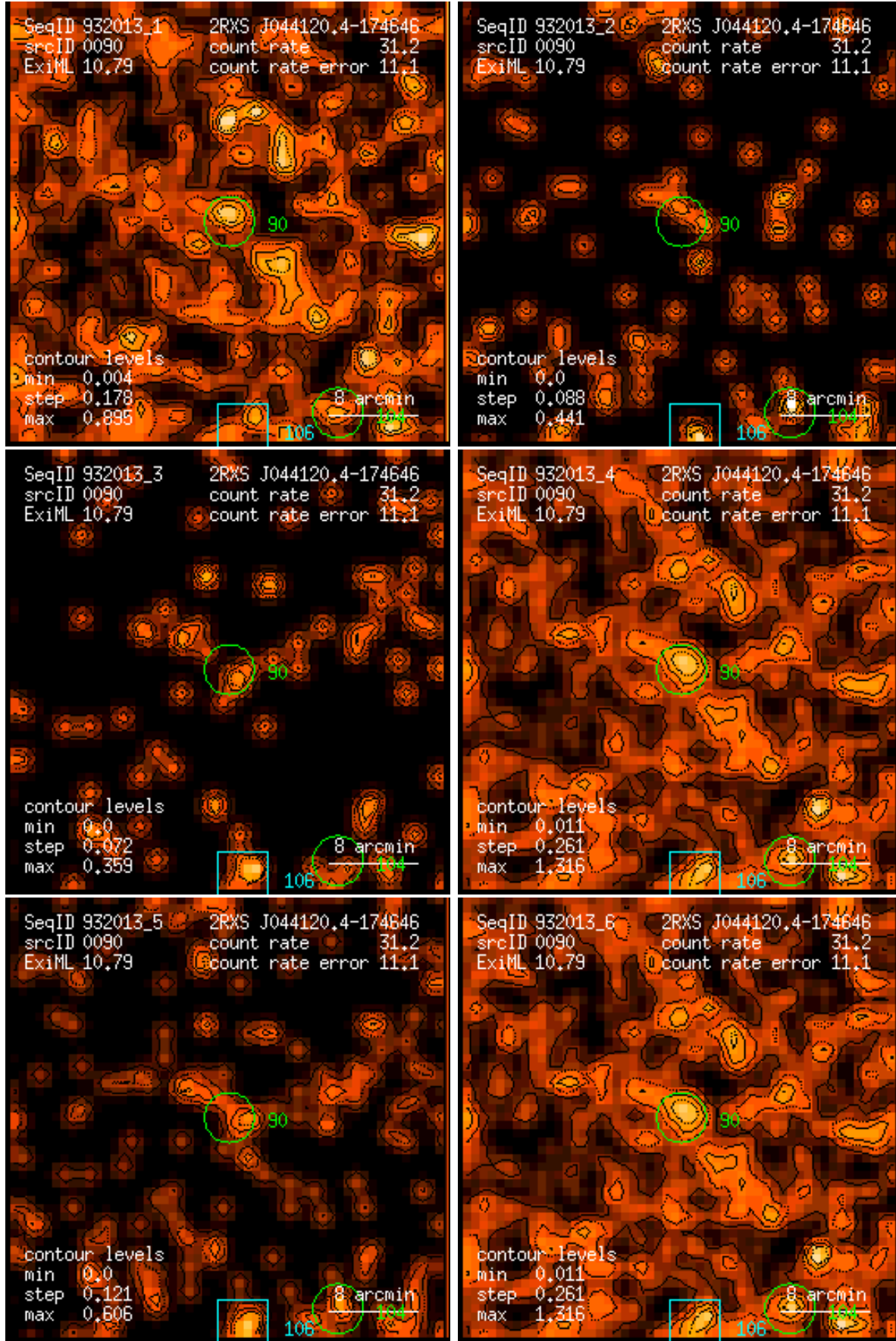
Figure 90: RASS 932013: detection 0090: band rate images, Gaussian filter: (1) PSPC channels 11 – 41, (2) 52 – 90, (3) 91 – 201, (4) 11 – 235, (5) 52 – 201, (6) 11 – 201. Broad band rates in counts/ks. Band rate contour levels in counts/ks/arcmin 2 .
