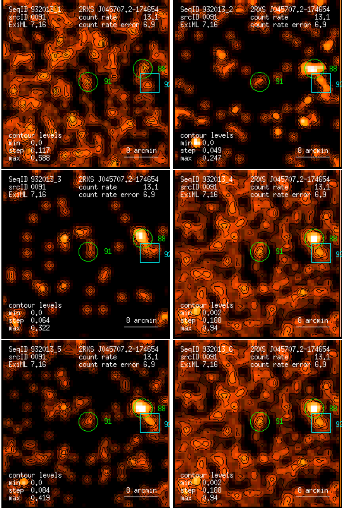
Figure 91: RASS 932013: detection 0091: band rate images, Gaussian filter: (1) PSPC channels 11 – 41, (2) 52 – 90, (3) 91 – 201, (4) 11 – 235, (5) 52 – 201, (6) 11 – 201. Broad band rates in counts/ks. Band rate contour levels in counts/ks/arcmin 2 .
