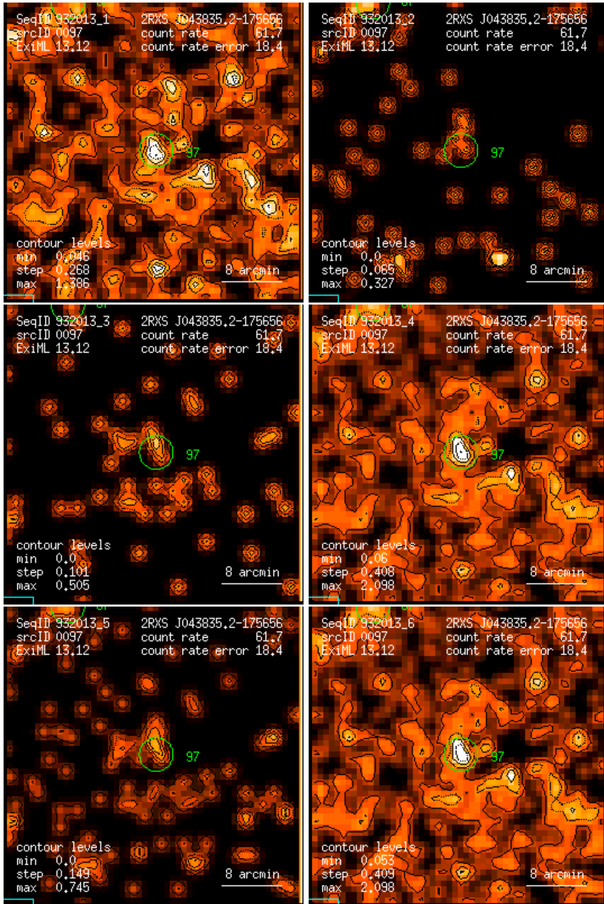
Figure 97: RASS 932013: detection 0097: band rate images, Gaussian filter: (1) PSPC channels 11 – 41, (2) 52 – 90, (3) 91 – 201, (4) 11 – 235, (5) 52 – 201, (6) 11 – 201. Broad band rates in counts/ks. Band rate contour levels in counts/ks/arcmin 2 .
