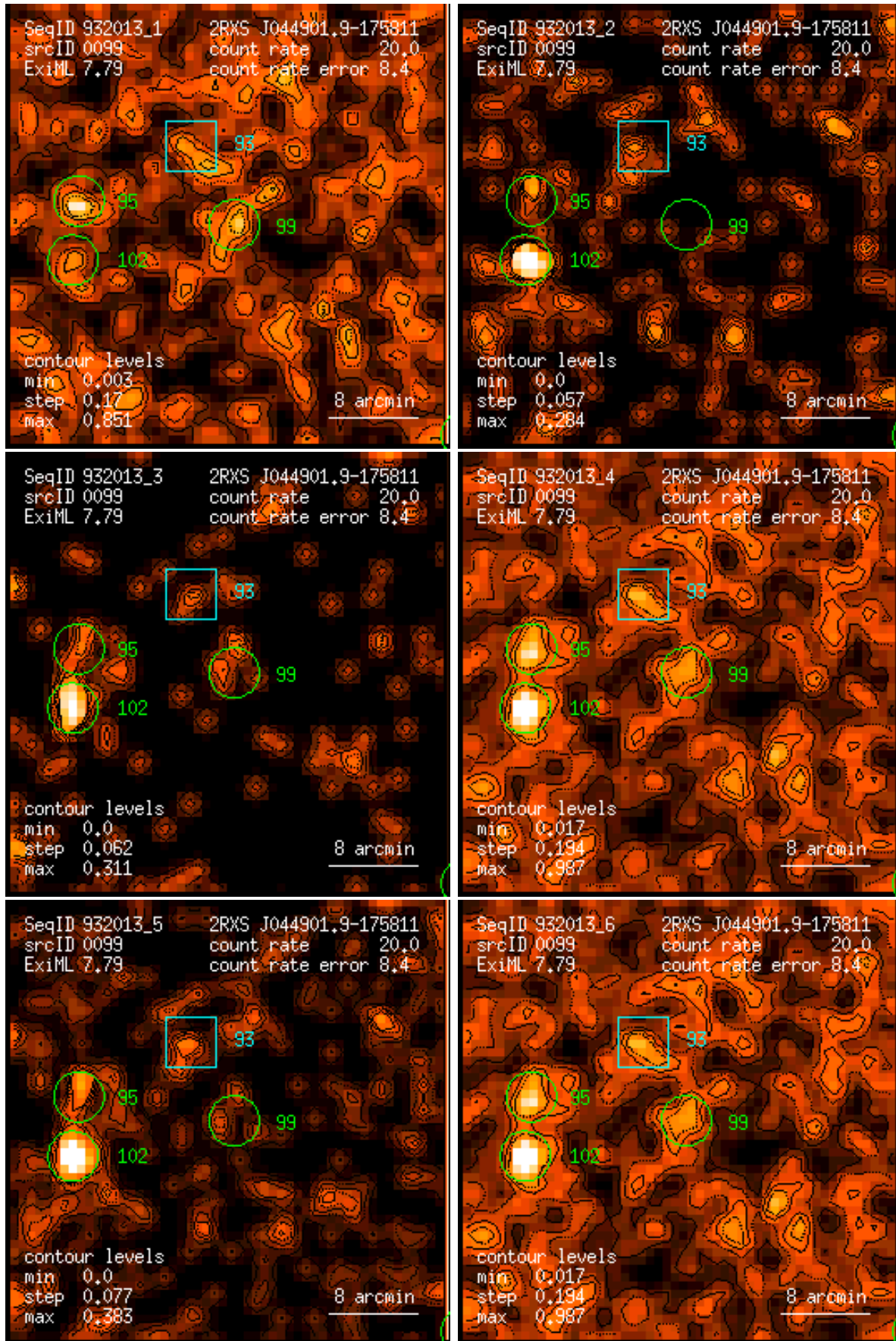
Figure 99: RASS 932013: detection 0099: band rate images, Gaussian filter: (1) PSPC channels 11 – 41, (2) 52 – 90, (3) 91 – 201, (4) 11 – 235, (5) 52 – 201, (6) 11 – 201. Broad band rates in counts/ks. Band rate contour levels in counts/ks/arcmin 2 .
